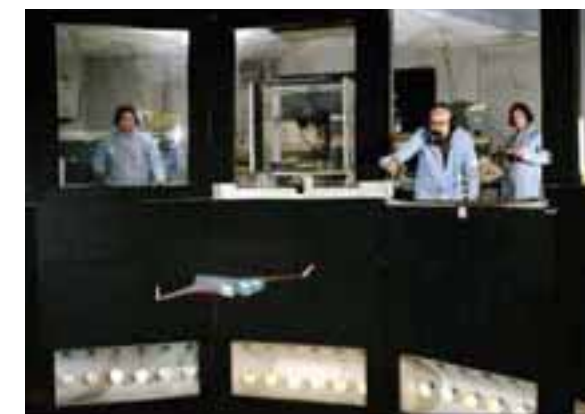
Free-spinning tests of a Blended Wing Body model in the Langley 20-Foot Vertical Spin Tunnel.
