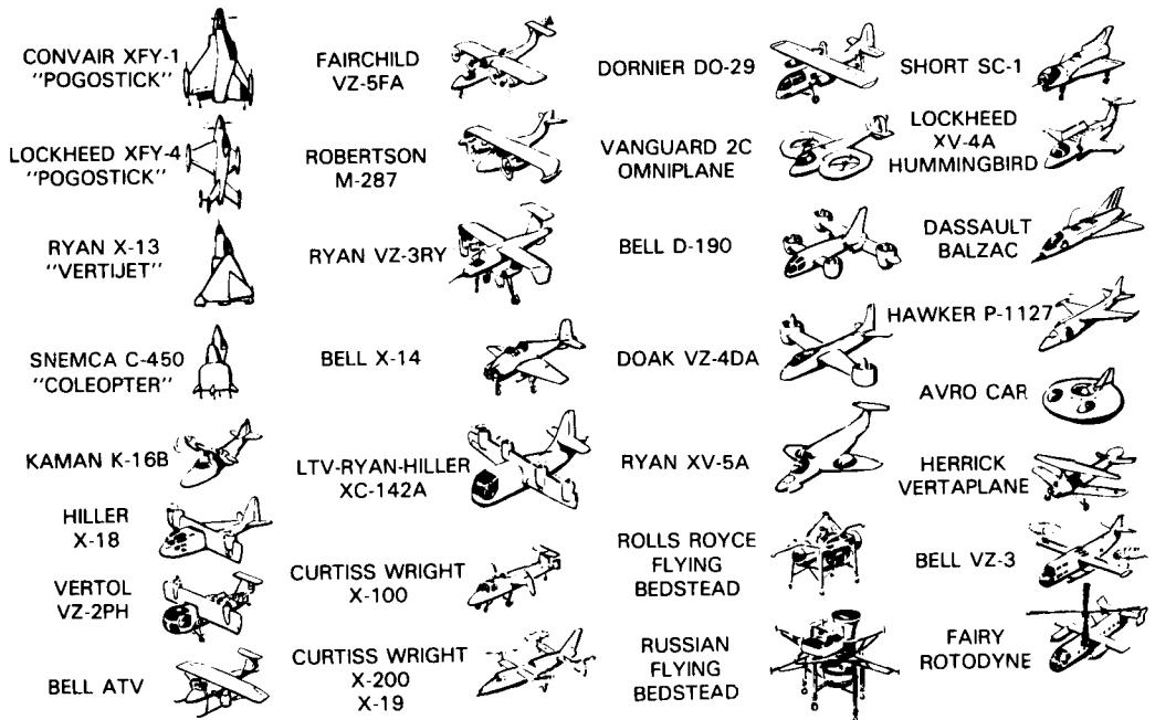
Figure 4-4. V/STOL Testbeds Analyzed by NASA
