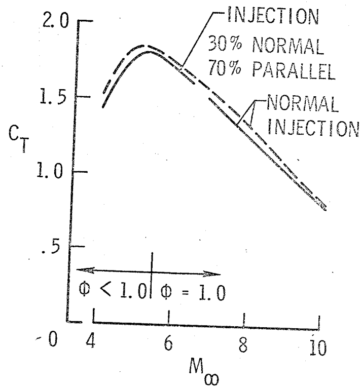
Figure 24.- Performance prediction.
