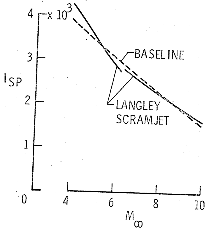
Figure 24.- Performance prediction.
