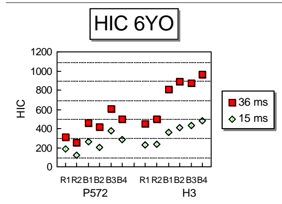
Figure 20 --6YO HIC values, Ford tests
