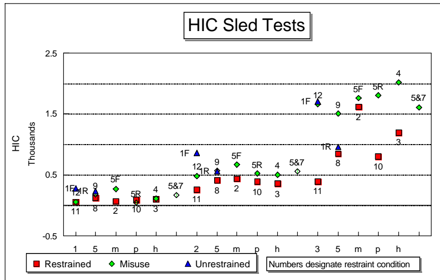
Figure 13 -- Kahane et al. HIC values
