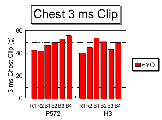
Figure 21 -- 6YO chest clips, Ford tests
