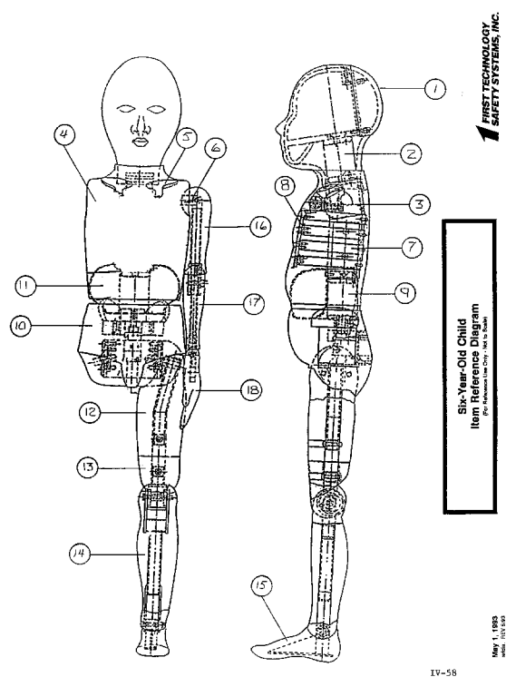
Figure 8 -- Part 572 6YO
