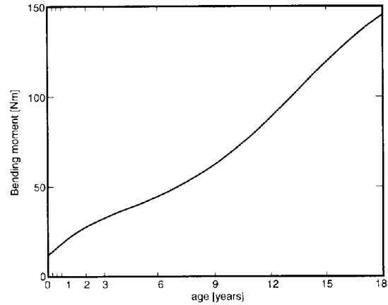
Figure 30 -- Janssen et al. scaled neck moment tolerances
