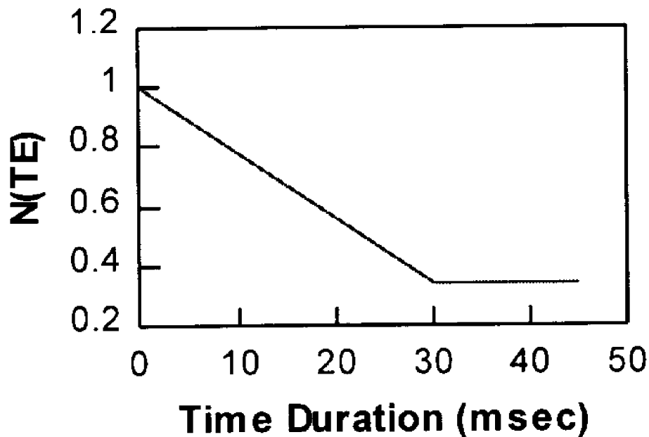
Figure 37 -- Neck tension/extension time duration requirement
