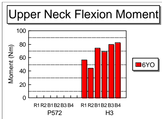
Figure 25 -- 6YO neck flexion, Ford tests
