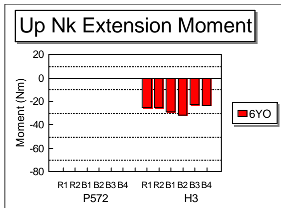
Figure 28 -- 6YO neck extension, Ford tests
