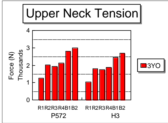
Figure 23 -- 3YO neck tension, Ford tests
