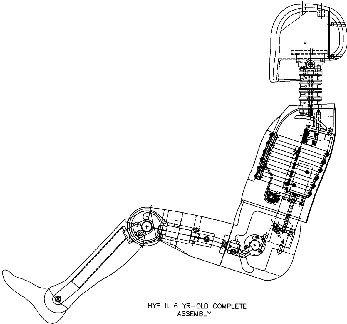
Figure 9 -- Hybrid III 6YO
