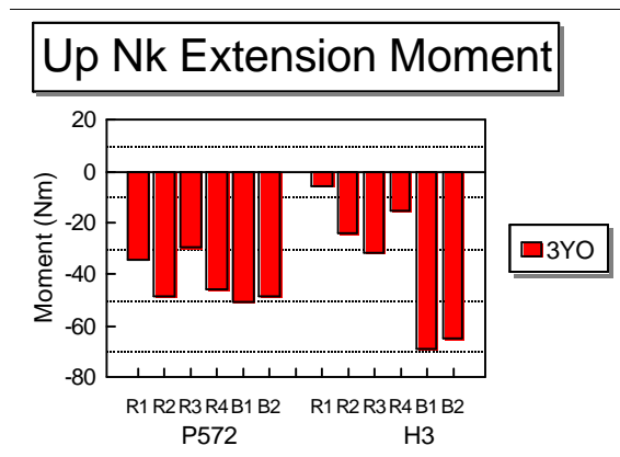
Figure 27 -- 3YO neck extension, Ford tests
