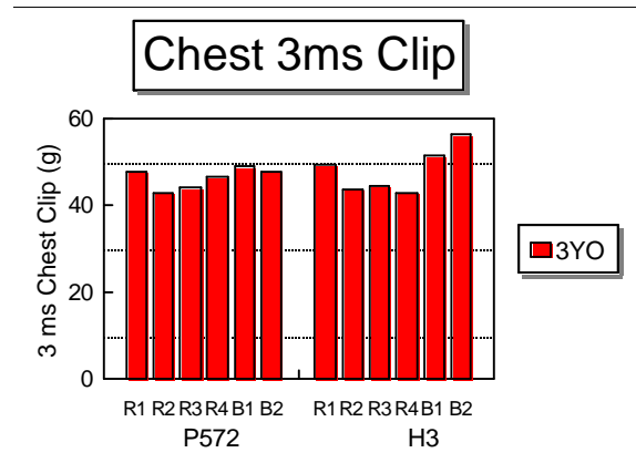
Figure 22 -- 3YO chest clips, Ford tests
