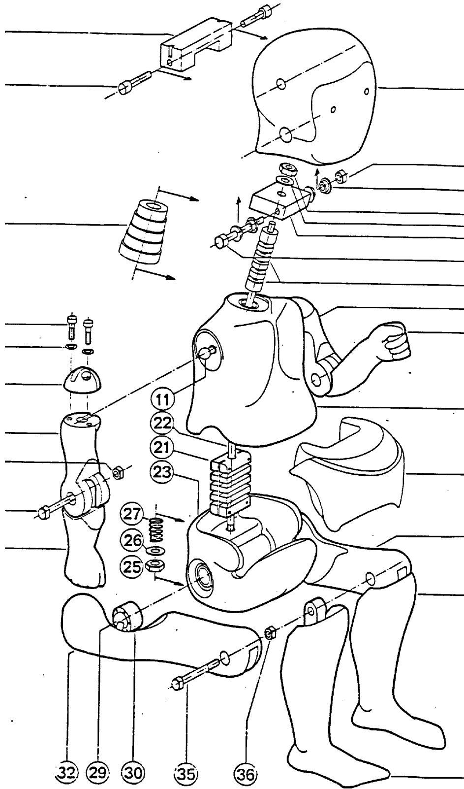
Figure 5 -- TNO dummy structure
