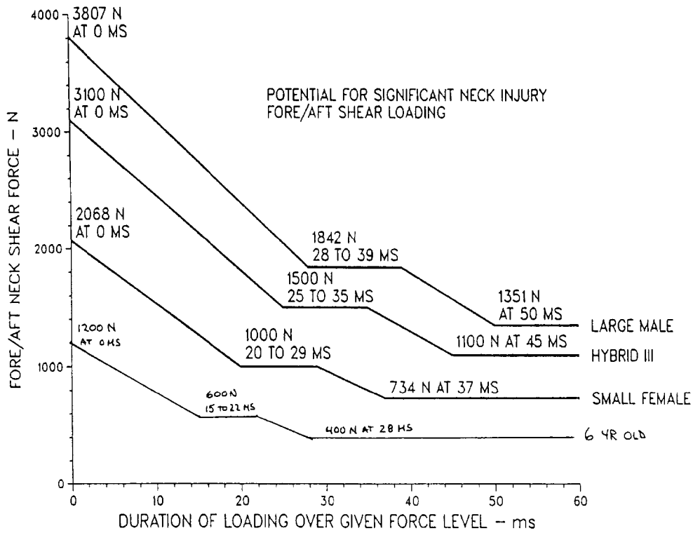
Figure 35 -- Fore/aft neck shear vs. Time duration (from GM IARV)
