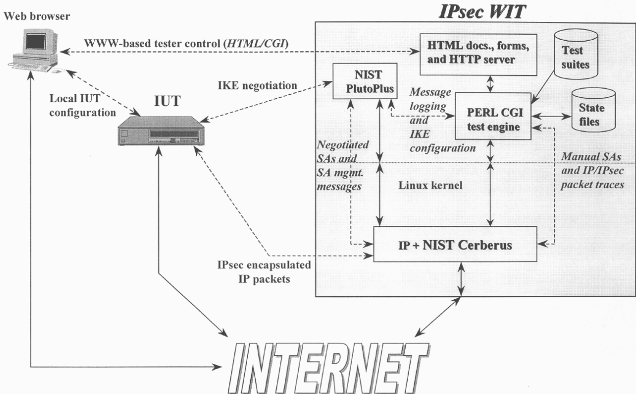
Fig. 5. IPsec-WIT architecture.
