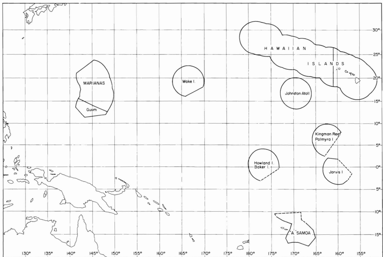
Figure 2.—Boundaries of the Fishery Conservation Zone around Hawaii, American Samoa, Guam, the Northern Mariana Islands, and other U.S. possessions.
