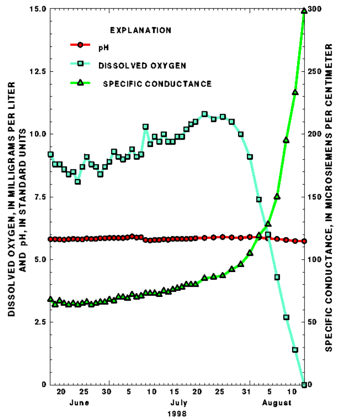
Figure 1. Ground-water quality measured by the automated monitoring process in well SDW 485-0102A, downgradient of the reactive wall, Cape Cod Massachusetts.
