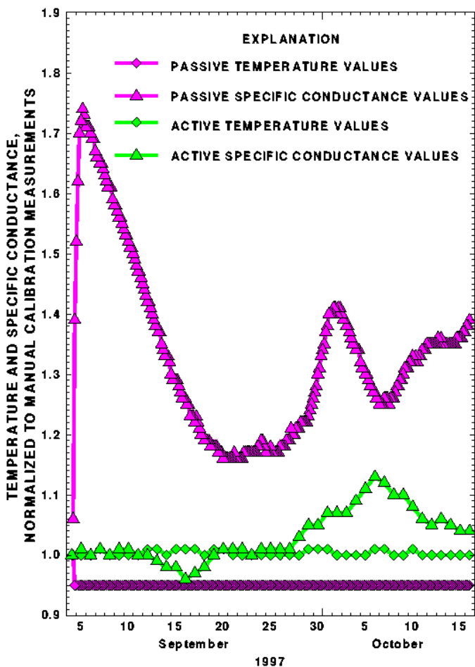
Figure 2. Normalized measurements of ground-water temperature and specific conductance by active and passive automated monitoring systems in wells SDW-0028 and SDW-0028A respectively.
