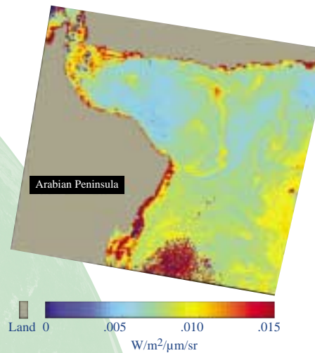
Chlorophyll Fluorescence Efficiency
