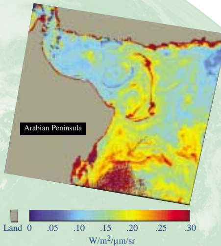
Fluorescence Line Height
