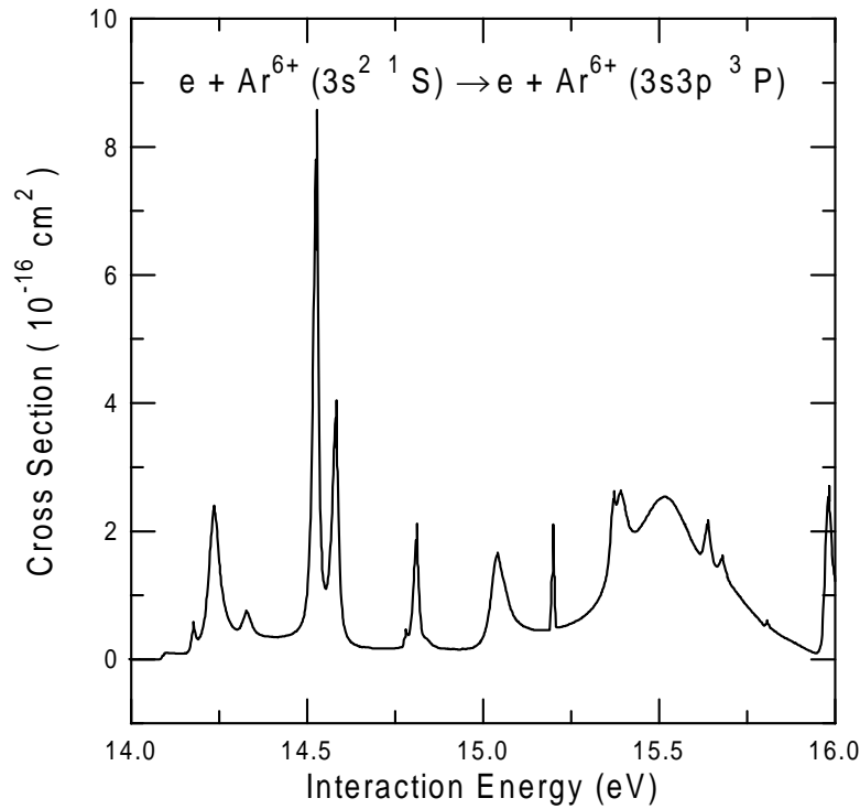
FIGURE 1. Cross sections for electron-impact excitation of the 3s^2 \ ^1S \rightarrow 3s3p \ ^3P transition in \text{Ar}^{6+} . The curve represents the close-coupling R-matrix calculations of Ref. 1. The small step at the threshold (14.1 eV in the calculation of Ref. 1) is the contribution of direct excitation.
