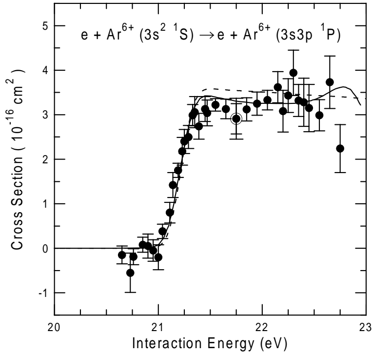
FIGURE 4. Cross sections for electron-impact excitation of the 3s^2 \ ^1S \rightarrow 3s3p \ ^1P transition in \text{Ar}^{6+} . The circles are the MEIBEL results of Ref. 17 with relative error bars at the 90% confidence level. The outer bars on the point at 21.75 eV represent the total expanded uncertainty. The solid curve is the 8-state CCR calculation of Ref. 1 convoluted with a 0.24 eV FWHM Gaussian representing the experimental energy distribution. The dashed curve is the DW calculation of Ref. 16 convoluted with the same Gaussian.
