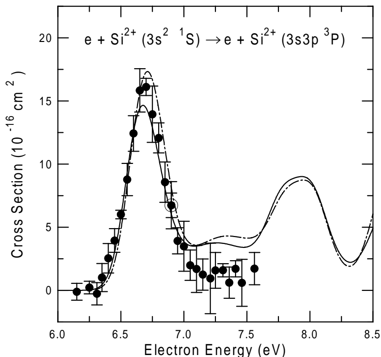
FIGURE 6. Cross sections for electron-impact excitation of the 3s^2\ ^1S \rightarrow 3s3p\ ^3P transition in \text{Si}^{2+} . The circles are the MEIBEL results of Ref. 18 with relative error bars at a 90% confidence level. The outer bars on the point at 6.9 eV represent the total expanded uncertainty. The curves are convolutions of a Gaussian (0.24 eV FWHM) with CCR calculations from Ref. 1 (solid) and Ref. 20 (dash-dot).
