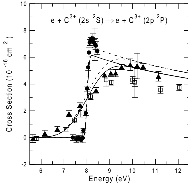
FIGURE 3. Cross sections for electron-impact excitation of the 2s \rightarrow 2p transition in C^{3+} . The circles represent the MEIBEL results of Ref. 14 and the triangles and squares the crossed-beams results of Refs. 13 and 7, respectively, with relative error bars at the 90% confidence level. The outer error bars on one point in each set represent the total expanded uncertainty. The solid curves are the 9-state CCR calculations of Ref. 15 convoluted with 0.17 eV and 1.7 eV FWHM Gaussians representing the energy distributions of Refs. 14 and 7, respectively. The dashed curves are the DW results of Ref. 16 convoluted with the same two Gaussians.
