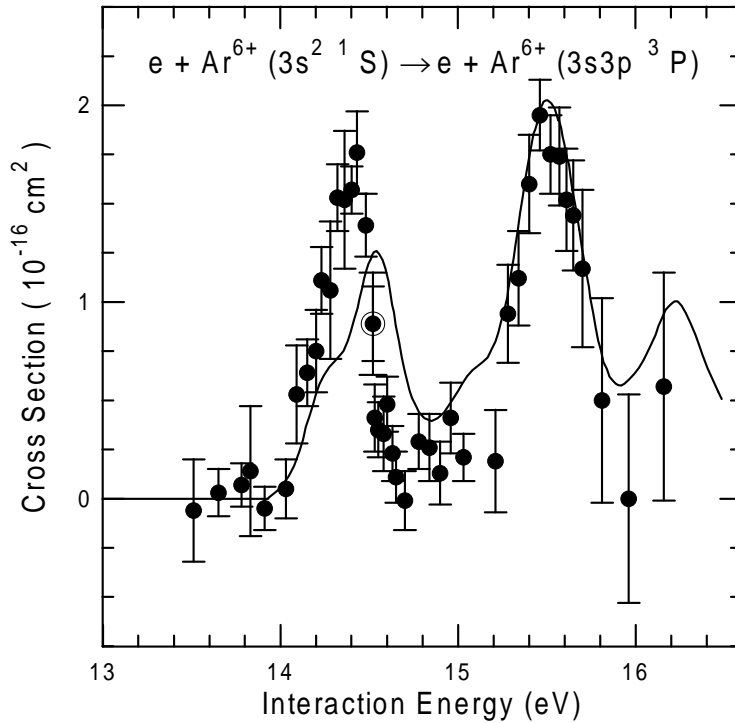
FIGURE 7. Cross sections for electron-impact excitation of the 3s^2\ ^1S \rightarrow 3s3p\ ^3P transition in \text{Ar}^{6+} . The circles are the MEIBEL results of Ref. 17 with relative error bars at a 90% confidence level. The outer bars on the point at 14.52 eV represent the total expanded uncertainty. The solid curve is a convolution of a Gaussian (0.24 eV FWHM) with CCR theory from Ref. 1.
