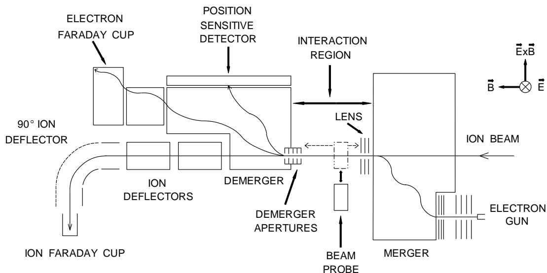
FIGURE 2. Schematic drawing of the JILA/ORNL merged electron-ion beams energy loss (MEIBEL) apparatus.
