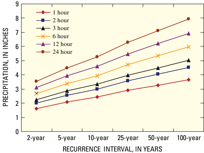
Figure 8. Precipitation-recurrence intervals for the Kansas City metropolitan area (modified from Young and McEnroe, 2006).
