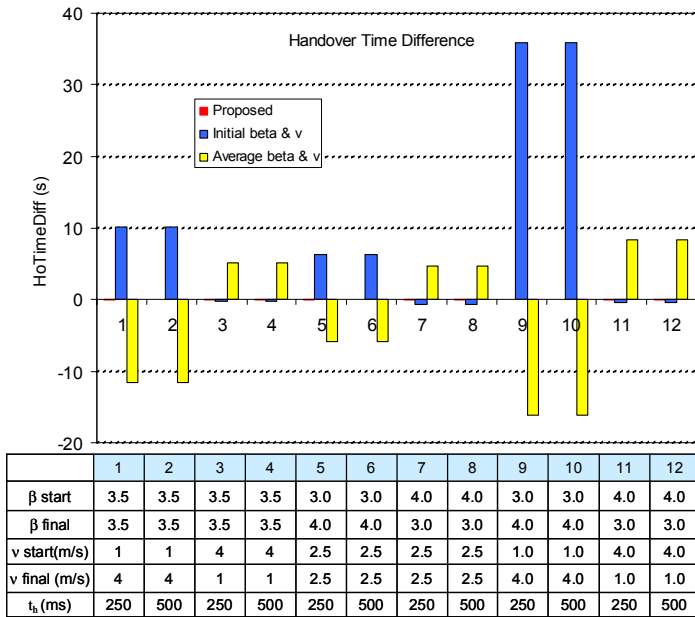
Figure 8. HoTimeDiff comparisons.
