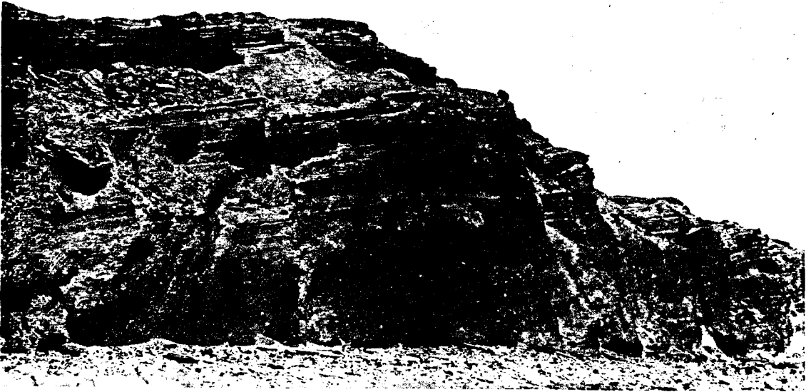
FIGURE 21.—Black Bluffs, east of the village, St. Paul Island.
