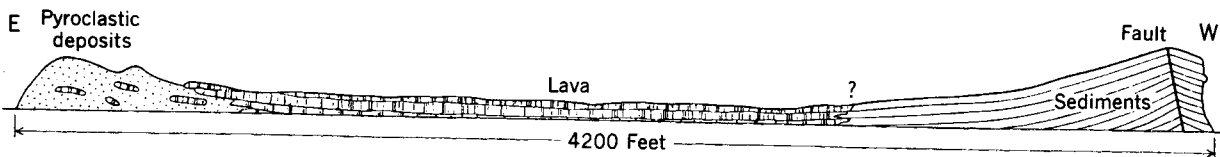
FIGURE 23.—Section of Otter Island. From east to west are pyroclastic rocks, lava, and sedimentary rocks.
