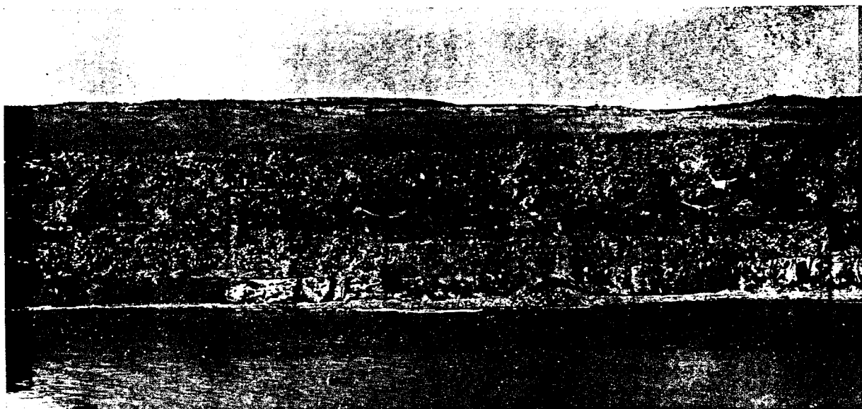
FIGURE 25.—Sea cliffs north of Garden Cove showing flows, sill and intercalated sediments (A) and overlying peridotite basement (B). Photograph by U. S. Navy.
