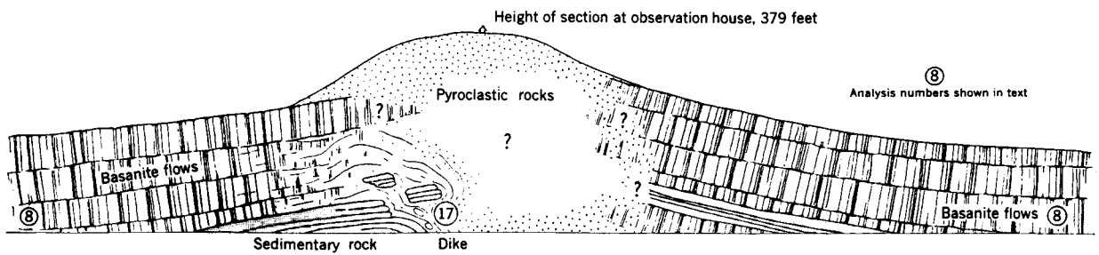
FIGURE 32.—Section through Einahnuhtu Bluffs, west coast of St. Paul Island.
