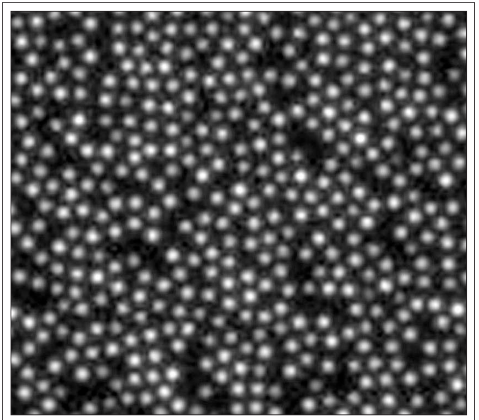
Fig. 5: A 1.2-mm square sample from a rear-illuminated projection screen.
