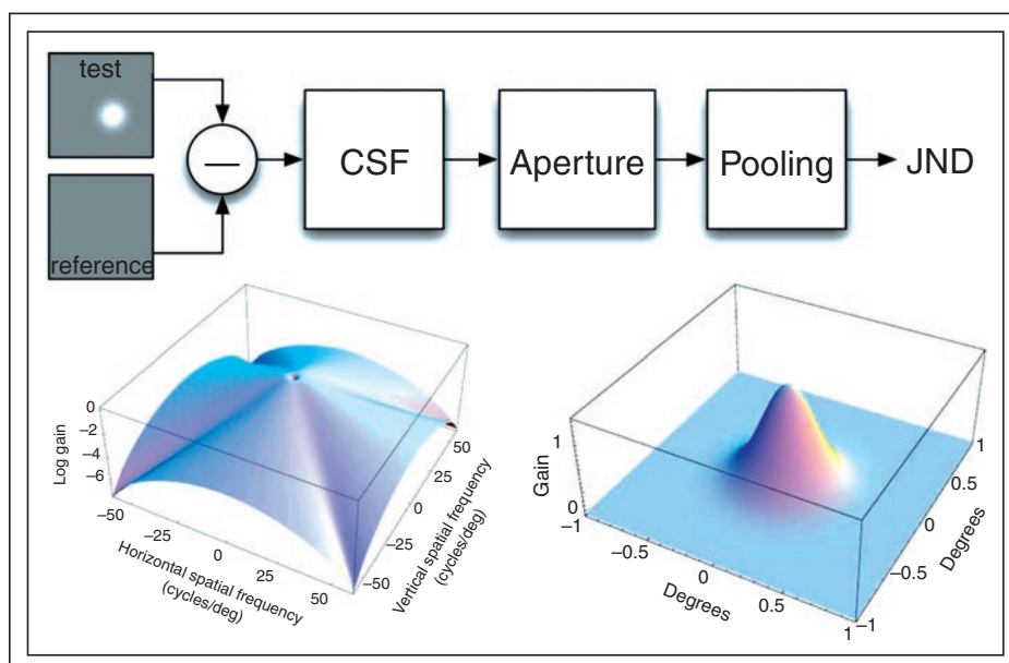
Fig. 1: Overview of the Spatial Standard Observer. The difference between test and reference images is filtered by a contrast-sensitivity function (CSF), windowed by an aperture function, and pooled non-linearly over space. The two graphs show the CSF (left) and the aperture (right).
