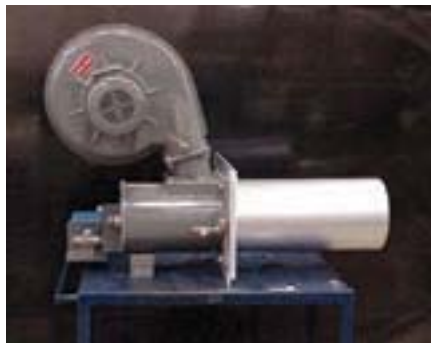
Figure 3. The Maxon MPAKT Ultra Low \text{NO}_x Burner is the first product that uses the ultra-clean low-swirl combustion technology.
