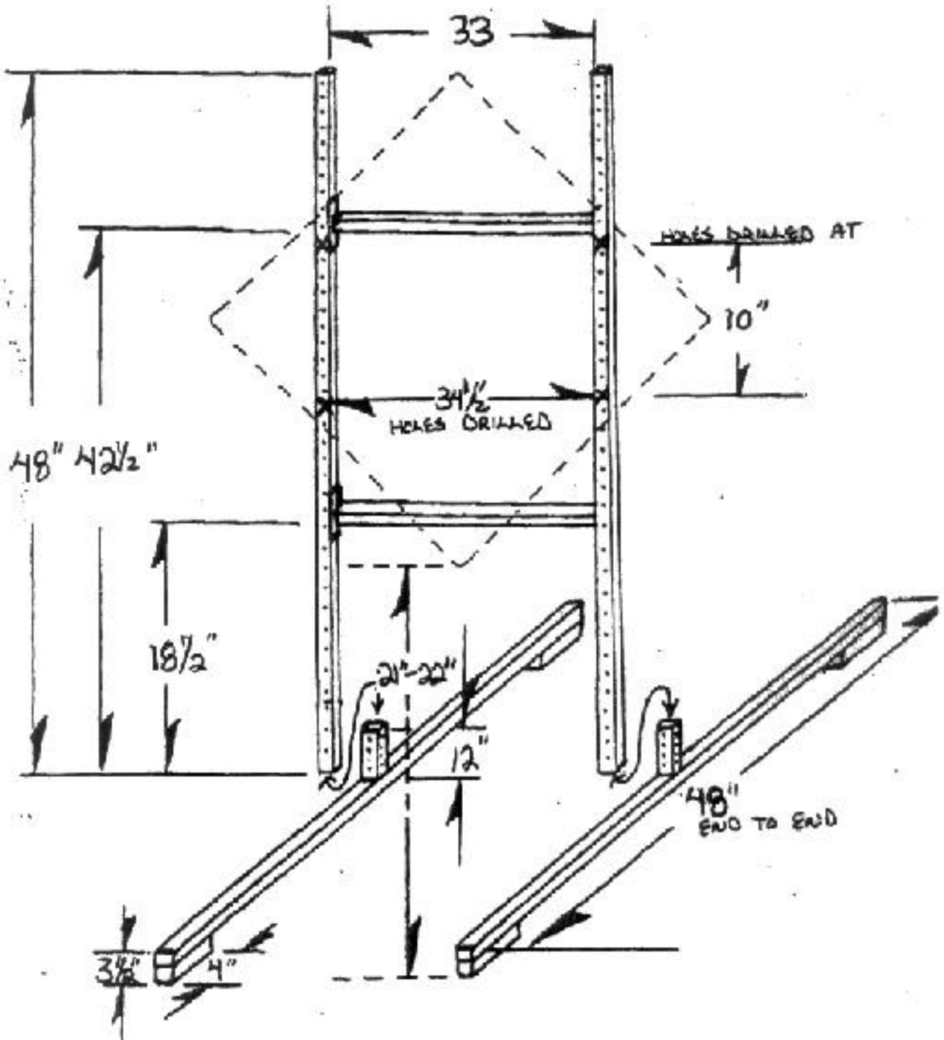
Illustration C-1. United Rentals Low H-stand Sign Stand (2 of 2)
