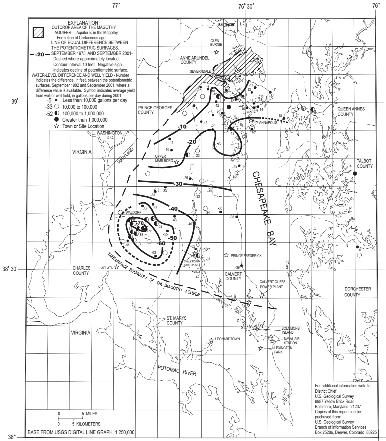
THE DIFFERENCE BETWEEN THE POTENTIOMETRIC SURFACES OF THE MAGOTHY AQUIFER, SEPTEMBER 1975 AND SEPTEMBER 2001 IN SOUTHERN MARYLAND
