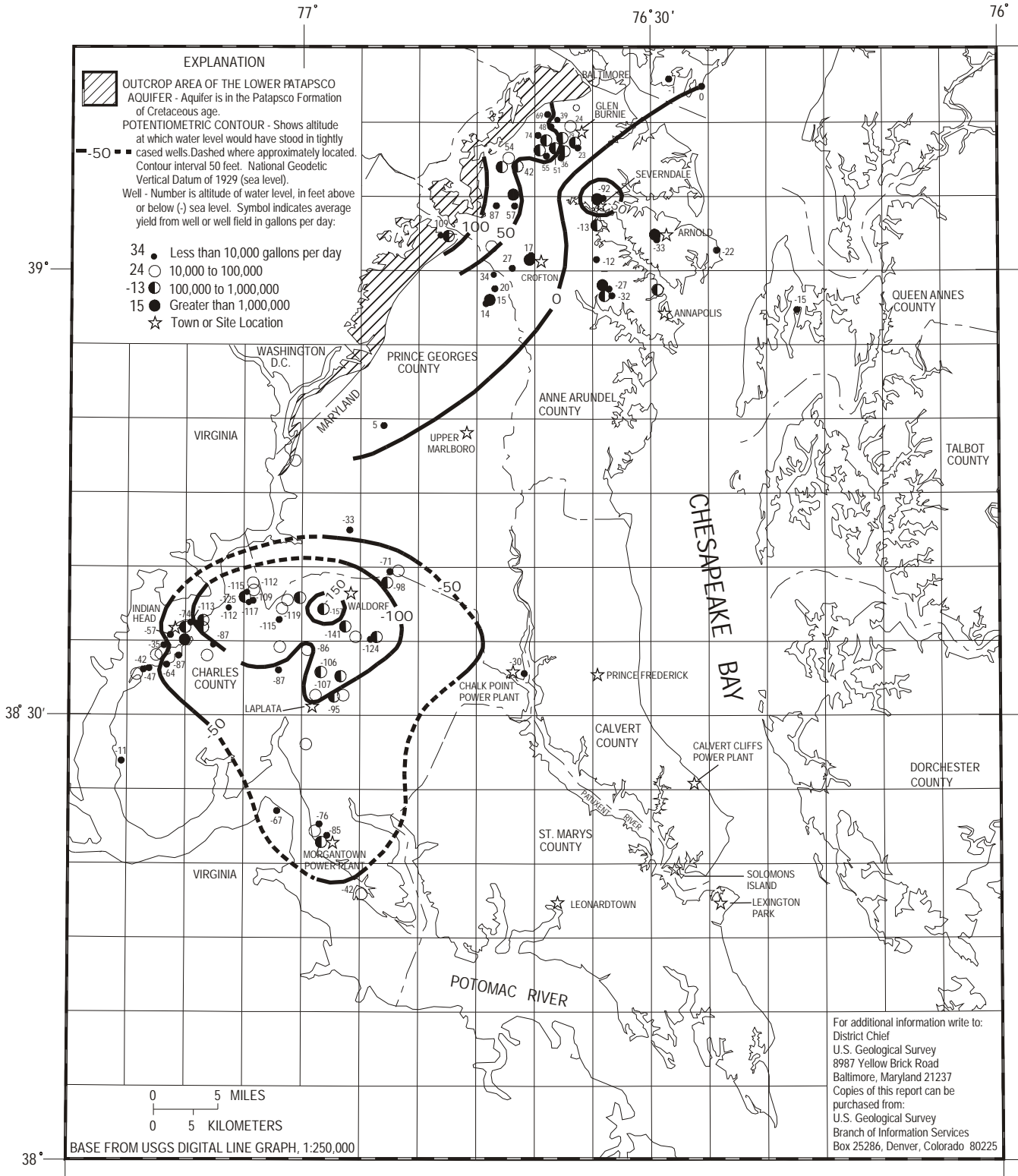
POTENTIOMETRIC SURFACE OF THE LOWER PATAPSCO AQUIFER IN SOUTHERN MARYLAND, SEPTEMBER 1999
