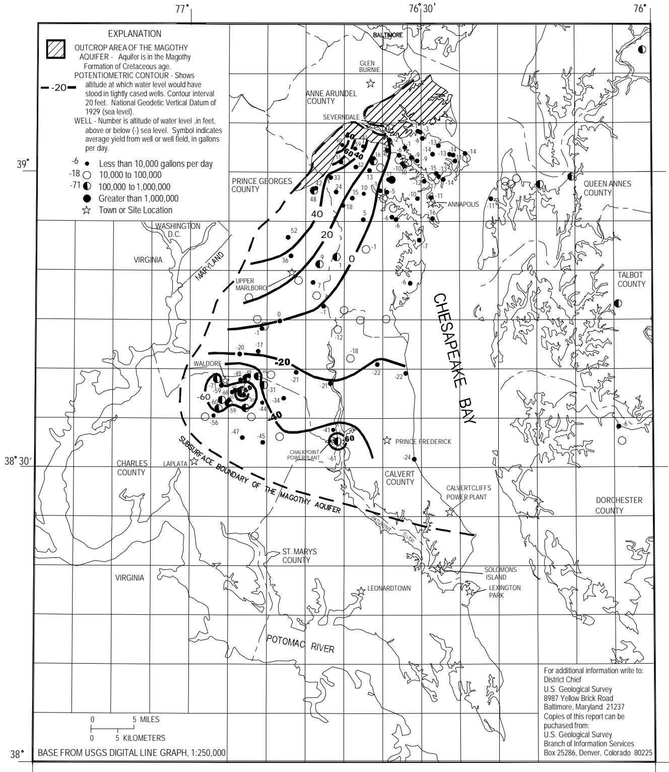
POTENTIOMETRIC SURFACE OF THE MAGOTHY AQUIFER IN SOUTHERN MARYLAND SEPTEMBER 1997
