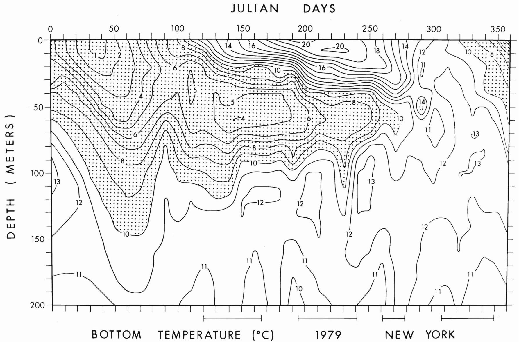
Appendix Figure 10.—Plot of bottom temperature (°C) on depth-time grid along the New York transect for 1979.
