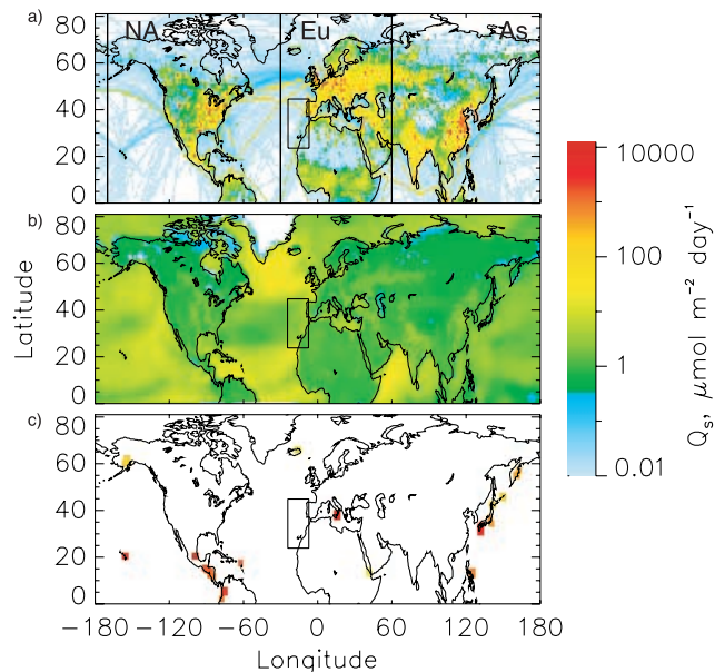
Figure 4. Sulfur emissions for the simulation period: (a) anthropogenic sources, (b) average biogenic sources, and (c) average volcanic sources. All panels use the scale shown. Volcanic emissions were divided by the area of the model grid cell where the volcano is located. The vertical lines in Figure 4a delimit the anthropogenic source regions distinguished in the model, North America (NA), Europe (Eu), and Asia (As). The rectangle delimits the ACE-2 experimental area ( 25^\circ – 8^\circ\text{W} longitude; 23^\circ – 44^\circ\text{N} latitude). See color version of this figure at back of this issue.
