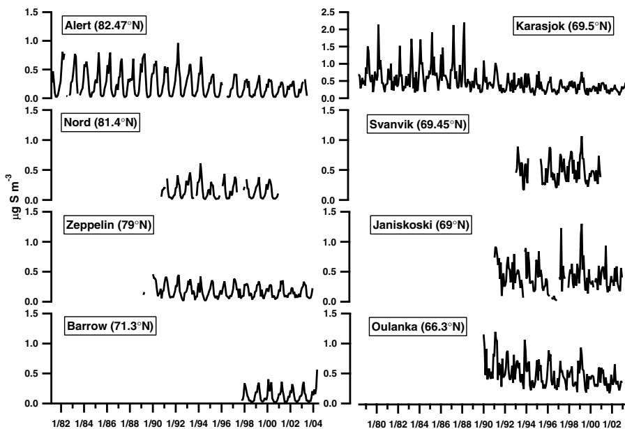
Fig. 2. Time-series of monthly averaged particulate sulphate concentrations in \mu\text{g S m}^{-3} for eight Arctic monitoring sites. Data made available for Alert by the Canadian National Atmospheric Chemistry (NAChem) Database and Analysis System, for Barrow by NOAA PMEL ( http://saga.pmel.noaa.gov/data/ ), and for the other stations by EMEP ( http://www.emep.int/ ).
