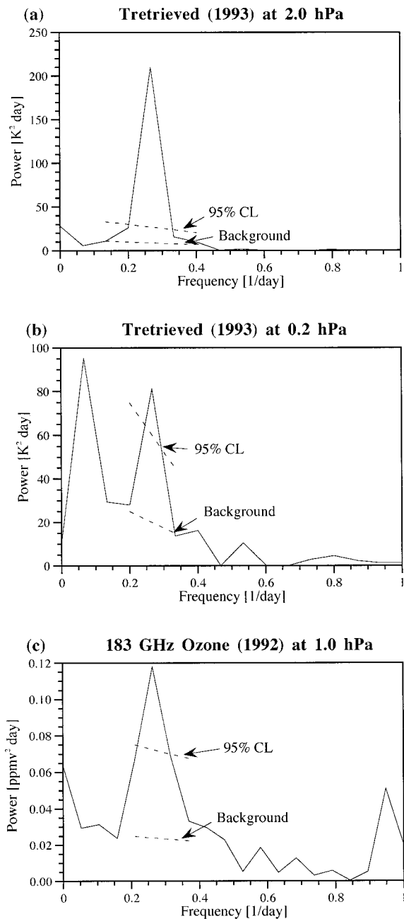
FIG. 9. Unsmoothed power spectra for wave 1 at 72^\circ\text{S} plotted along with estimated background and 95% confidence level. (a) T_{\text{retrieved}} for the 1993 series at 2 hPa. (b) T_{\text{retrieved}} for the 1993 series at 0.2 hPa. (c) 183-GHz ozone for the 1992 series at 1.0 hPa.
