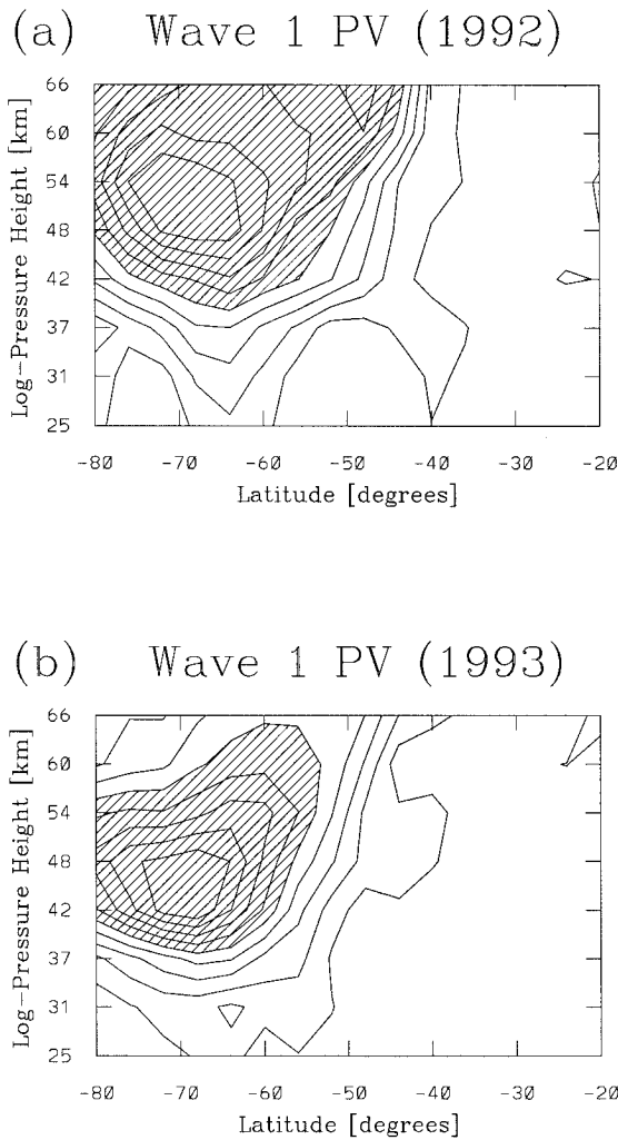
FIG. 13. (a) Quasigeostrophic potential vorticity amplitude for wave 1 and 3.8-day eastward period for 18 August–6 September 1992. (b) Same as (a) but for 2–16 September 1993, 3.75-day period. Contours are at every 10% interval of the maximum with values higher than 50% shaded.
