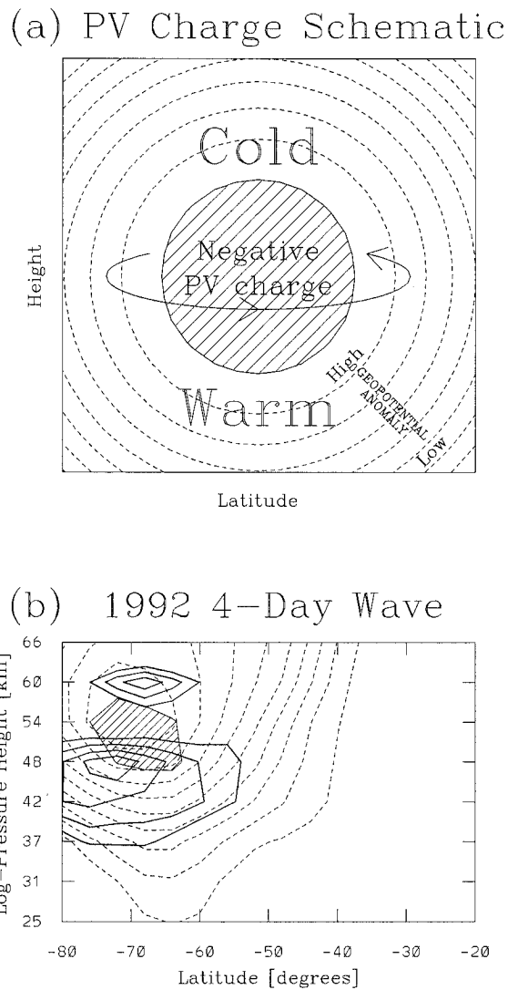
FIG. 14. (a) “PV charge” schematic adapted from Bishop and Thorpe (1994), Figs. 1 and 2. The negative PV anomaly induces temperature, geopotential, and wind (solid line with arrows) anomalies as shown. Note: the PV, temperature, and geopotential anomalies are viewed here as a meridional cross section of the three-dimensional PV charge, while the circulation is in a horizontal plane that projects out of the page. (b) Amplitude of wave 1, 3.8-day eastward period signal from 18 August to 6 September 1992. Hatched region includes PV amplitude greater than 90% of the maximum. Solid lines are perturbation temperature amplitude of 60%–90%, incremented by 10% of the maximum. Dashed lines are perturbation geopotential amplitude at every 10% of the maximum. Adapted from Figs. 4a, 6a, and 13a of this paper.
