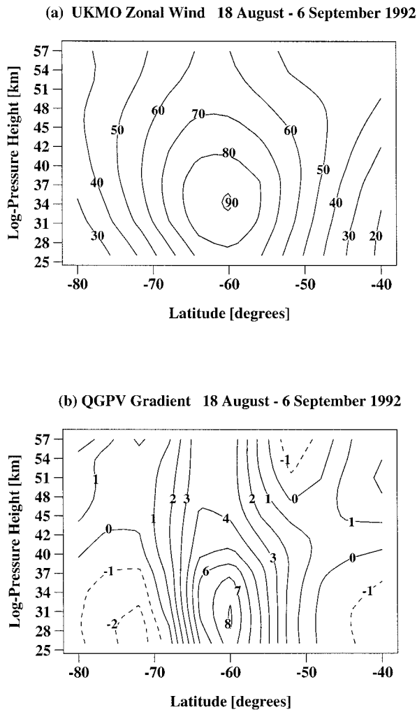
FIG. 10. (a) UKMO zonal mean zonal wind (westerly, in \text{m s}^{-1} ) averaged from 18 August to 6 September 1992. (b) Quasigeostrophic potential vorticity gradient, \bar{q}_y , averaged from 18 August to 6 September 1992. Contour increment is 1.0 \times 10^{-11} \text{m}^{-1} \text{s}^{-1} with negative values dashed.
