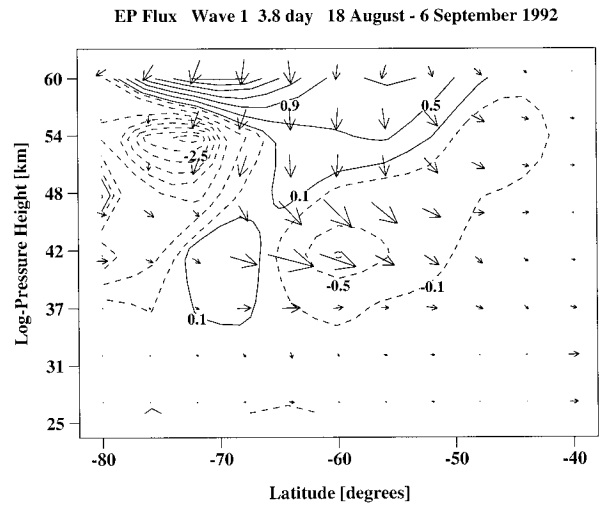
FIG. 11. Eliassen–Palm flux diagram calculated for the wave 1, 3.8-day eastward period components of MLS temperature and geopotential height from 18 August to 6 September 1992. Contours are DF = \nabla \cdot \mathbf{F} / (\rho_0 a \cos \phi) starting at 0.1 and incremented at 0.4 \text{ m s}^{-1} \text{ day}^{-1} with solid (dashed) line indicating positive (negative) values. Arrows are the Eliassen–Palm flux vectors.
