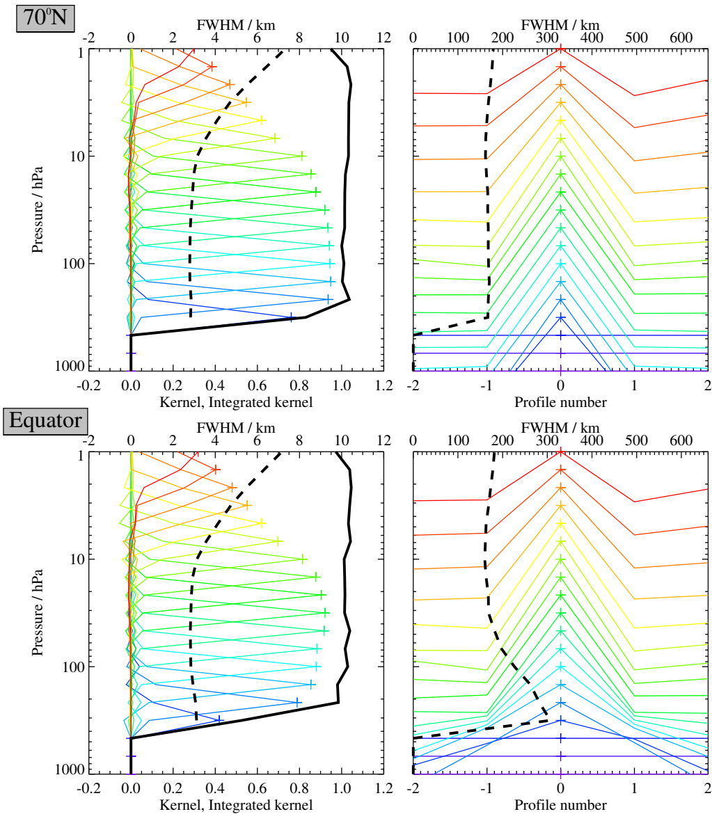
Figure 3.24: Typical two-dimensional (vertical and horizontal along-track) averaging kernels for the MLS v2.2 SO 2 data at 70°N (upper) and the equator (lower); variation in the averaging kernels is sufficiently small that these are representative of typical profiles. Colored lines show the averaging kernels as a function of MLS retrieval level, indicating the region of the atmosphere from which information is contributing to the measurements on the individual retrieval surfaces, which are denoted by plus signs in corresponding colors. The dashed black line indicates the resolution, determined from the full width at half maximum (FWHM) of the averaging kernels, approximately scaled into kilometers (top axes). (Left) Vertical averaging kernels (integrated in the horizontal dimension for five along-track profiles) and resolution. The solid black line shows the integrated area under each kernel (horizontally and vertically); values near unity imply that the majority of information for that MLS data point has come from the measurements, whereas lower values imply substantial contributions from a priori information. (Right) Horizontal averaging kernels (integrated in the vertical dimension) and resolution. The averaging kernels are scaled such that a unit change is equivalent to one decade in pressure.
