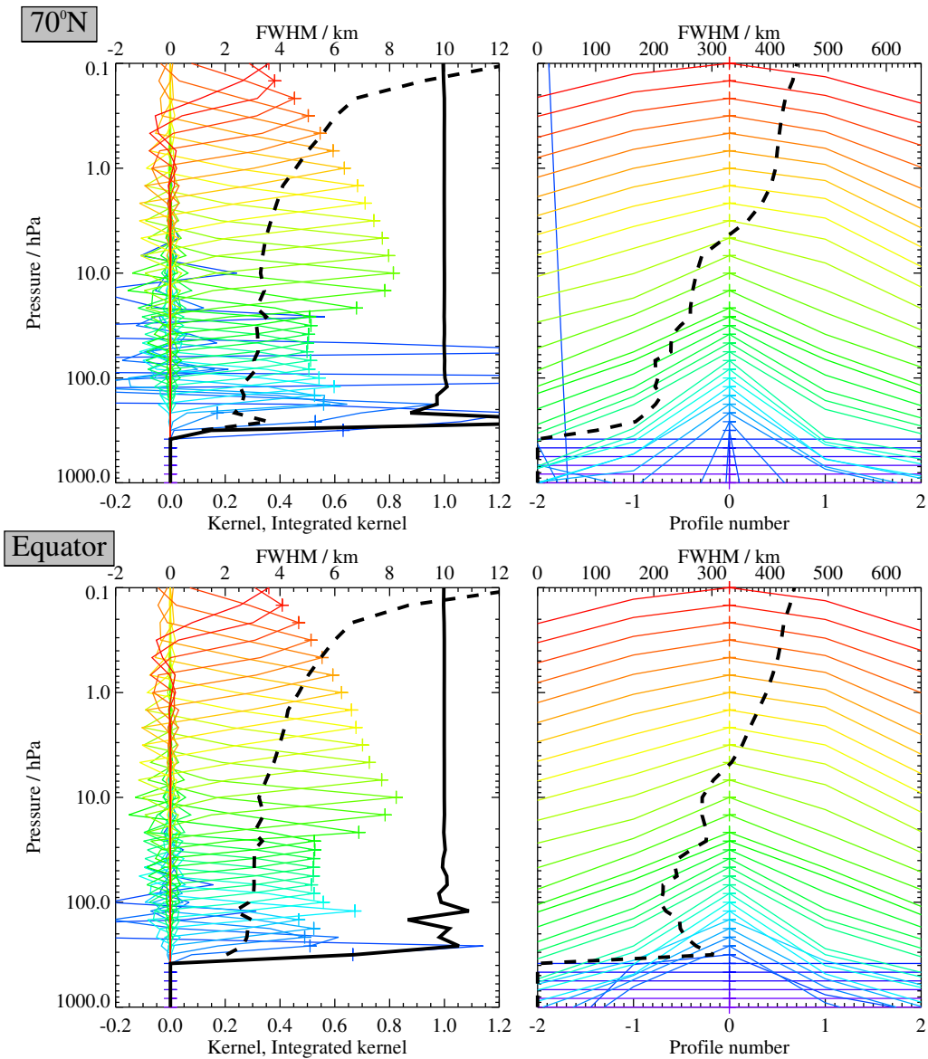
Figure 3.8: Typical two-dimensional (vertical and horizontal along-track) averaging kernels for the MLS v2.2 H 2 O data at 70°N (upper) and the equator (lower); variation in the averaging kernels is sufficiently small that these are representative of typical profiles. Colored lines show the averaging kernels as a function of MLS retrieval level, indicating the region of the atmosphere from which information is contributing to the measurements on the individual retrieval surfaces, which are denoted by plus signs in corresponding colors. The dashed black line indicates the resolution, determined from the full width at half maximum (FWHM) of the averaging kernels, approximately scaled into kilometers (top axes). (Left) Vertical averaging kernels (integrated in the horizontal dimension for five along-track profiles) and resolution. The solid black line shows the integrated area under each kernel (horizontally and vertically); values near unity imply that the majority of information for that MLS data point has come from the measurements, whereas lower values imply substantial contributions from a priori information. (Right) Horizontal averaging kernels (integrated in the vertical dimension) and resolution. The averaging kernels are scaled such that a unit change is equivalent to one decade in pressure.
