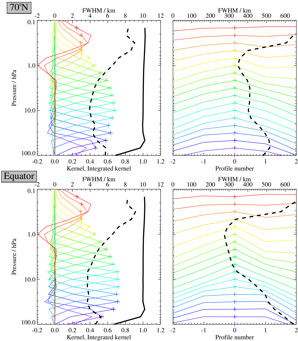
Figure 3.19: Typical two-dimensional (vertical and horizontal along-track) averaging kernels for the MLS v2.2 N_2O data at 70^\circ N (upper) and the equator (lower); variation in the averaging kernels is sufficiently small that these are representative of typical profiles. Colored lines show the averaging kernels as a function of MLS retrieval level, indicating the region of the atmosphere from which information is contributing to the measurements on the individual retrieval surfaces, which are denoted by plus signs in corresponding colors. The dashed black line indicates the resolution, determined from the full width at half maximum (FWHM) of the averaging kernels, approximately scaled into kilometers (top axes). (Left) Vertical averaging kernels (integrated in the horizontal dimension for five along-track profiles) and resolution. The solid black line shows the integrated area under each kernel (horizontally and vertically); values near unity imply that the majority of information for that MLS data point has come from the measurements, whereas lower values imply substantial contributions from a priori information. (Right) Horizontal averaging kernels (integrated in the vertical dimension) and resolution. The averaging kernels are scaled such that a unit change is equivalent to one decade in pressure.
