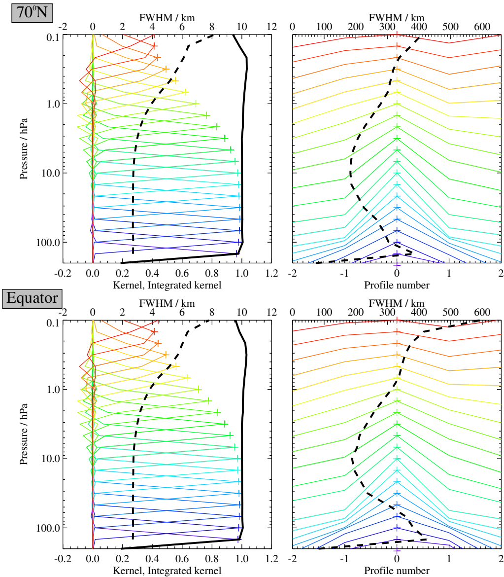
Figure 3.9: Typical two-dimensional (vertical and horizontal along-track) averaging kernels for the MLS v2.2 HCI data at 70°N (upper) and the equator (lower); variation in the averaging kernels is sufficiently small that these are representative of typical profiles. Colored lines show the averaging kernels as a function of MLS retrieval level, indicating the region of the atmosphere from which information is contributing to the measurements on the individual retrieval surfaces, which are denoted by plus signs in corresponding colors. The dashed black line indicates the resolution, determined from the full width at half maximum (FWHM) of the averaging kernels, approximately scaled into kilometers (top axes). (Left) Vertical averaging kernels (integrated in the horizontal dimension for five along-track profiles) and resolution. The solid black line shows the integrated area under each kernel (horizontally and vertically); values near unity imply that the majority of information for that MLS data point has come from the measurements, whereas lower values imply substantial contributions from a priori information. (Right) Horizontal averaging kernels (integrated in the vertical dimension) and resolution. The averaging kernels are scaled such that a unit change is equivalent to one decade in pressure.
