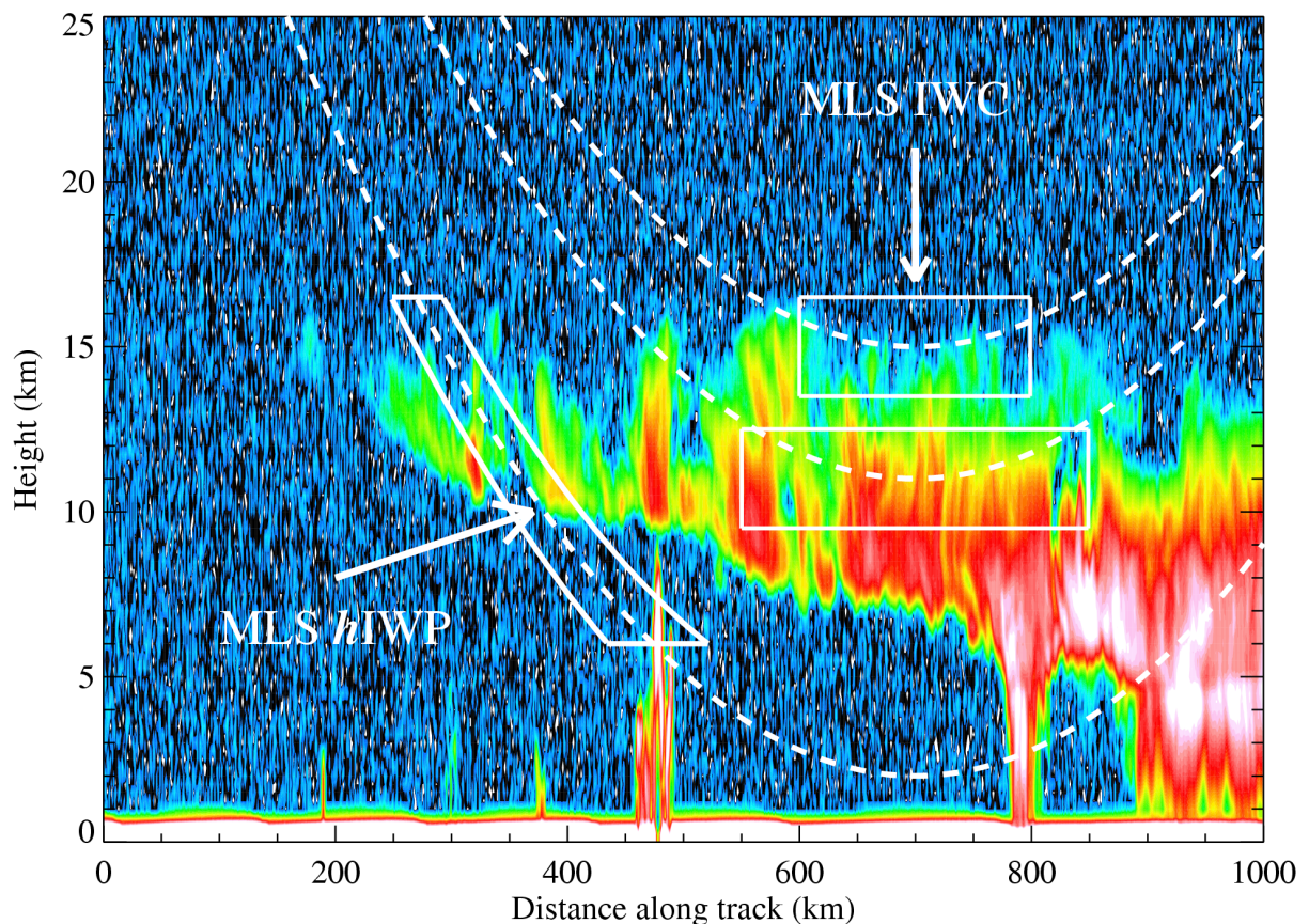
Figure 3.18: Diagram to illustrate the MLS IWC and IWP measurement. The dashed lines are the MLS tangential beams. At high tangent heights, the beams penetrate through the limb and become sensitive to a volume-averaged IWC, whereas at low tangent heights the MLS beams cannot penetrate through the limb due to strong gaseous absorption and become only sensitive to a partial column of IWP, namely, hIWP, with a shallow angle ( \sim 3^\circ ). The slant path of IWP, or hIWP, has a 3^\circ elevation angle. Note that the actual volume of the hIWP locates at \sim 300 km away from the tangent point, or \sim 2 profiles from the location of the nominal profile.
