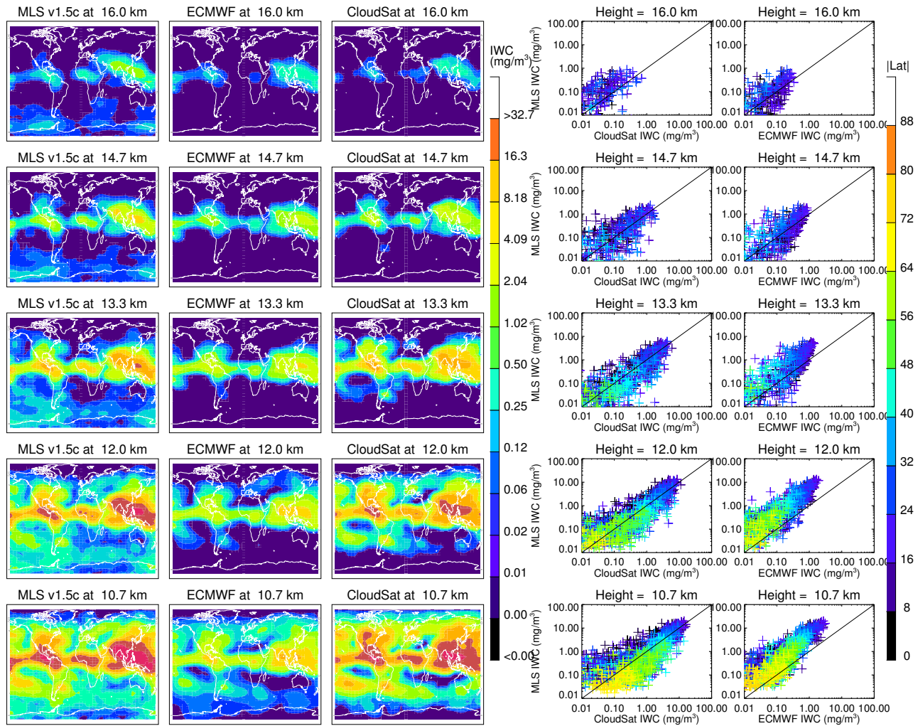
Figure 3.17: Maps on left show MLS, ECMWF, and CloudSat IWC maps at 215–100 hPa for the period 7 July–16 August, 2006. The pressure levels (215, 177, 147, 121, 100 hPa) correspond to nominal altitudes of 10.7, 12, 13.3, 14.7, and 16 km approximately. All maps share the same color scale and have the same 4^\circ \times 8^\circ lat-lon grid. For ECMWF and CloudSat maps, the vertical resolution is reduced to 3 km with further binning to match the MLS vertical resolution. On the right are the scatter plots of grid-averaged IWC values from the maps, where color denotes latitude from the equator and the 1:1 ratio is added as a guide.
