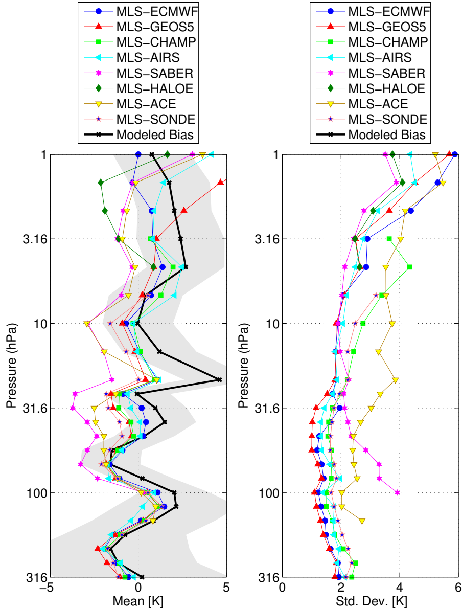
Figure 3.26: The left panel shows globally-averaged mean differences between MLS temperature and eight correlative data sets. Criteria for coincidences are described in detail in Schwartz et al. [2007]. The right panel shows the global standard deviations about the means. The dark green line is
