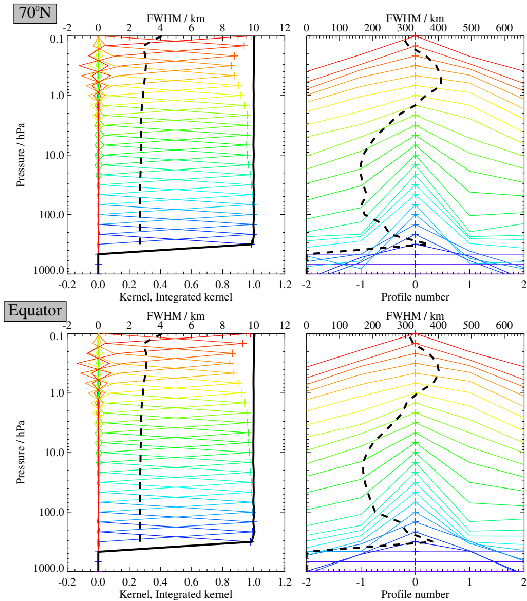
Figure 3.21: Typical two-dimensional (vertical and horizontal along-track) averaging kernels for the MLS v2.2 O 3 data at 70°N (upper) and the equator (lower); variation in the averaging kernels is sufficiently small that these are representative of typical profiles. Colored lines show the averaging kernels as a function of MLS retrieval level, indicating the region of the atmosphere from which information is contributing to the measurements on the individual retrieval surfaces, which are denoted by plus signs in corresponding colors. The dashed black line indicates the resolution, determined from the full width at half maximum (FWHM) of the averaging kernels, approximately scaled into kilometers (top axes). (Left) Vertical averaging kernels (integrated in the horizontal dimension for five along-track profiles) and resolution. The solid black line shows the integrated area under each kernel (horizontally and vertically); values near unity imply that the majority of information for that MLS data point has come from the measurements, whereas lower values imply substantial contributions from a priori information. (Right) Horizontal averaging kernels (integrated in the vertical dimension) and resolution. The averaging kernels are scaled such that a unit change is equivalent to one decade in pressure.
