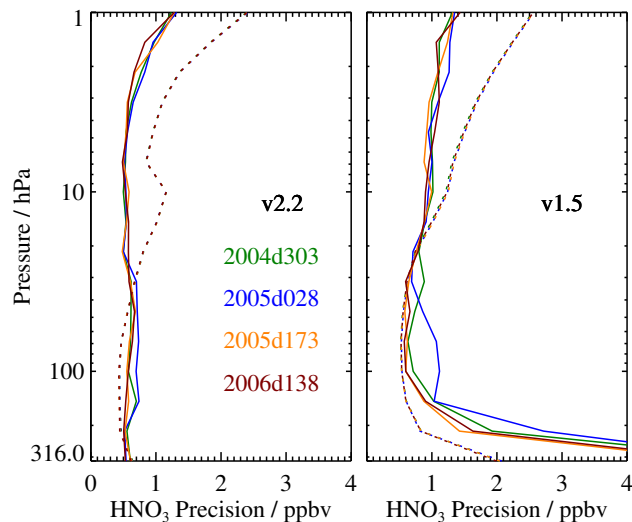
Figure 3.13: Precision of the (left) v2.2 and (right) v1.5 MLS HNO 3 measurements for four representative days (see legend). Solid lines depict the observed scatter in a narrow equatorial band (see text); dotted lines depict the theoretical precision estimated by the retrieval algorithm.
