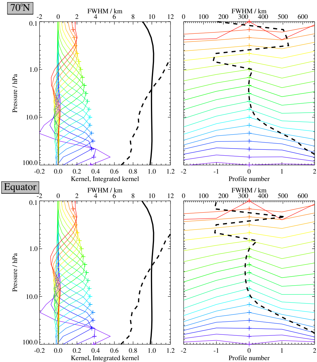
Figure 3.10: Typical two-dimensional (vertical and horizontal along-track) averaging kernels for the MLS v2.2 HCN data at 70°N (upper) and the equator (lower); variation in the averaging kernels is sufficiently small that these are representative of typical profiles. Colored lines show the averaging kernels as a function of MLS retrieval level, indicating the region of the atmosphere from which information is contributing to the measurements on the individual retrieval surfaces, which are denoted by plus signs in corresponding colors. The dashed black line indicates the resolution, determined from the full width at half maximum (FWHM) of the averaging kernels, approximately scaled into kilometers (top axes). (Left) Vertical averaging kernels (integrated in the horizontal dimension for five along-track profiles) and resolution. The solid black line shows the integrated area under each kernel (horizontally and vertically); values near unity imply that the majority of information for that MLS data point has come from the measurements, whereas lower values imply substantial contributions from a priori information. (Right) Horizontal averaging kernels (integrated in the vertical dimension) and resolution. The averaging kernels are scaled such that a unit change is equivalent to one decade in pressure.
