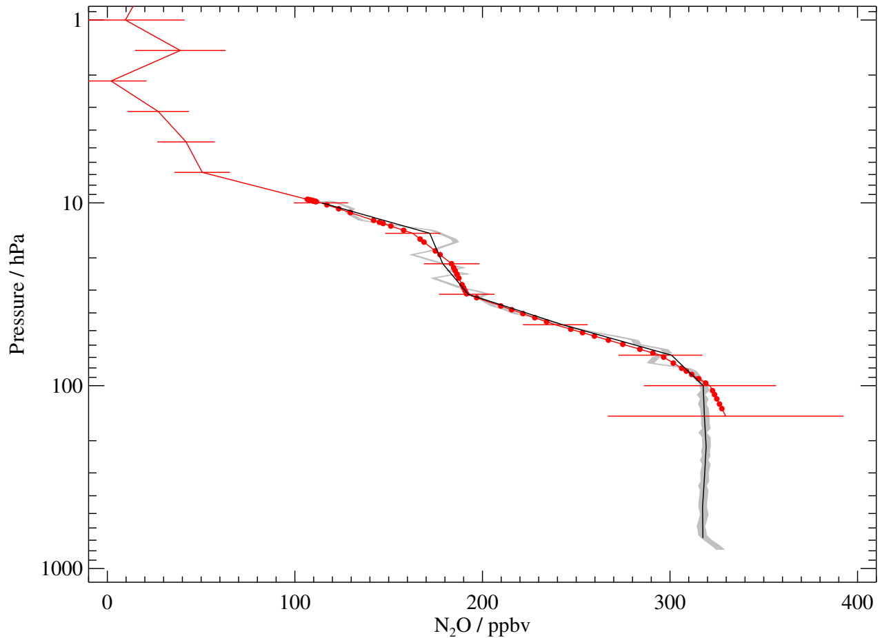
Figure 1.2: Comparisons of MLS (v1.5) N 2 O observations with in-situ balloon data (courtesy of J. Elkins). The raw balloon data ( \mathbf{z}_h ) are shown as the grey shaded region (shading indicates precision). A coincident MLS profile ( \mathbf{x}_l ) is shown in red with the red error bars indicating precision. The red dots show the MLS data linearly interpolated to the balloon pressures using the \mathbf{H} matrix (i.e., \mathbf{x}_h from equation 1.1). The black line shows the ‘least squares’ interpolation of the balloon data onto the MLS grid using the \mathbf{W} matrix as described in the text (i.e., \mathbf{z}_l from equation 1.2). The black line therefore represents the closest possible match at this resolution to the original grey line, and is the appropriate quantity to compare to the red MLS profile.
