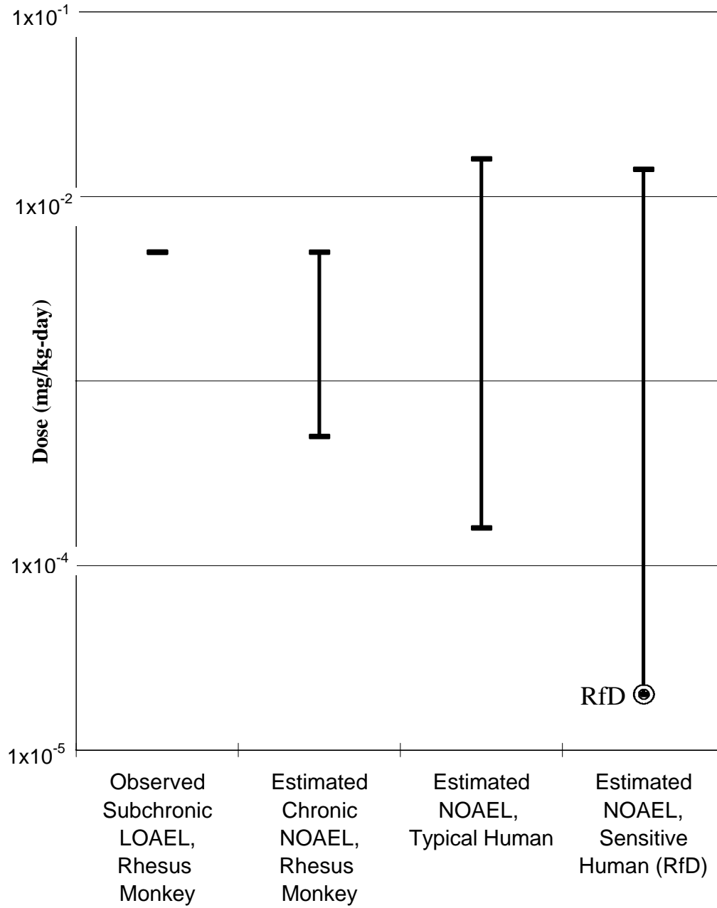
Figure 4-1: Results of Tryphonas et al. (1989) and the Cumulative Uncertainty in the RfD for Aroclor 1254
