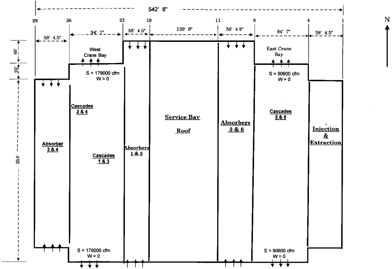
Figure 1 3rd Floor Plan – Building 9201-5
