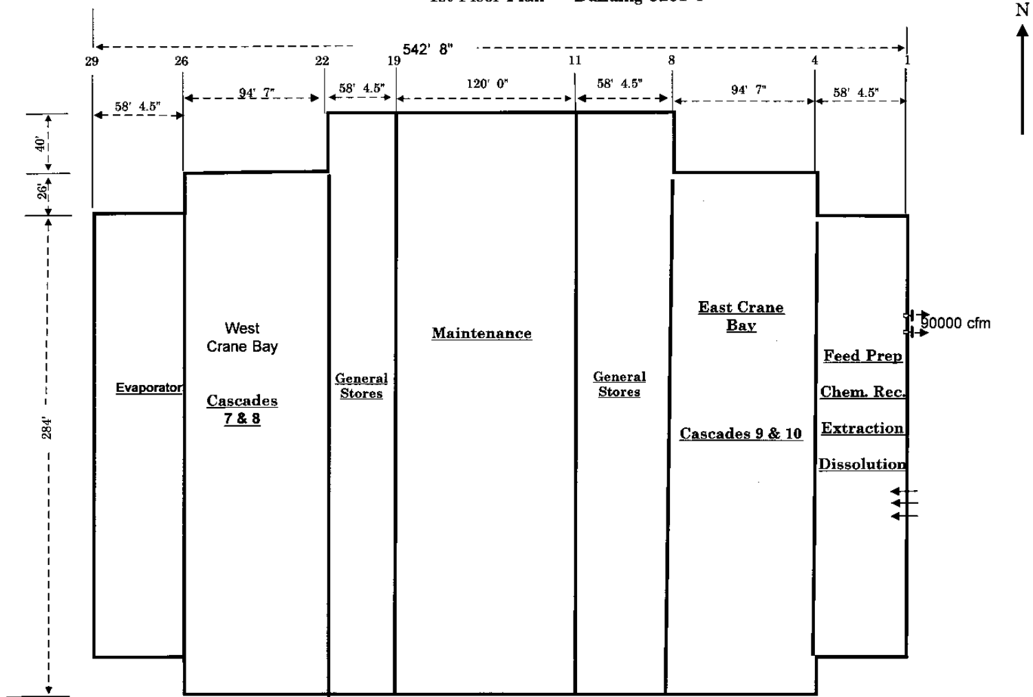
Figure 1 "1st Floor Plan" -- Building 9201-4
