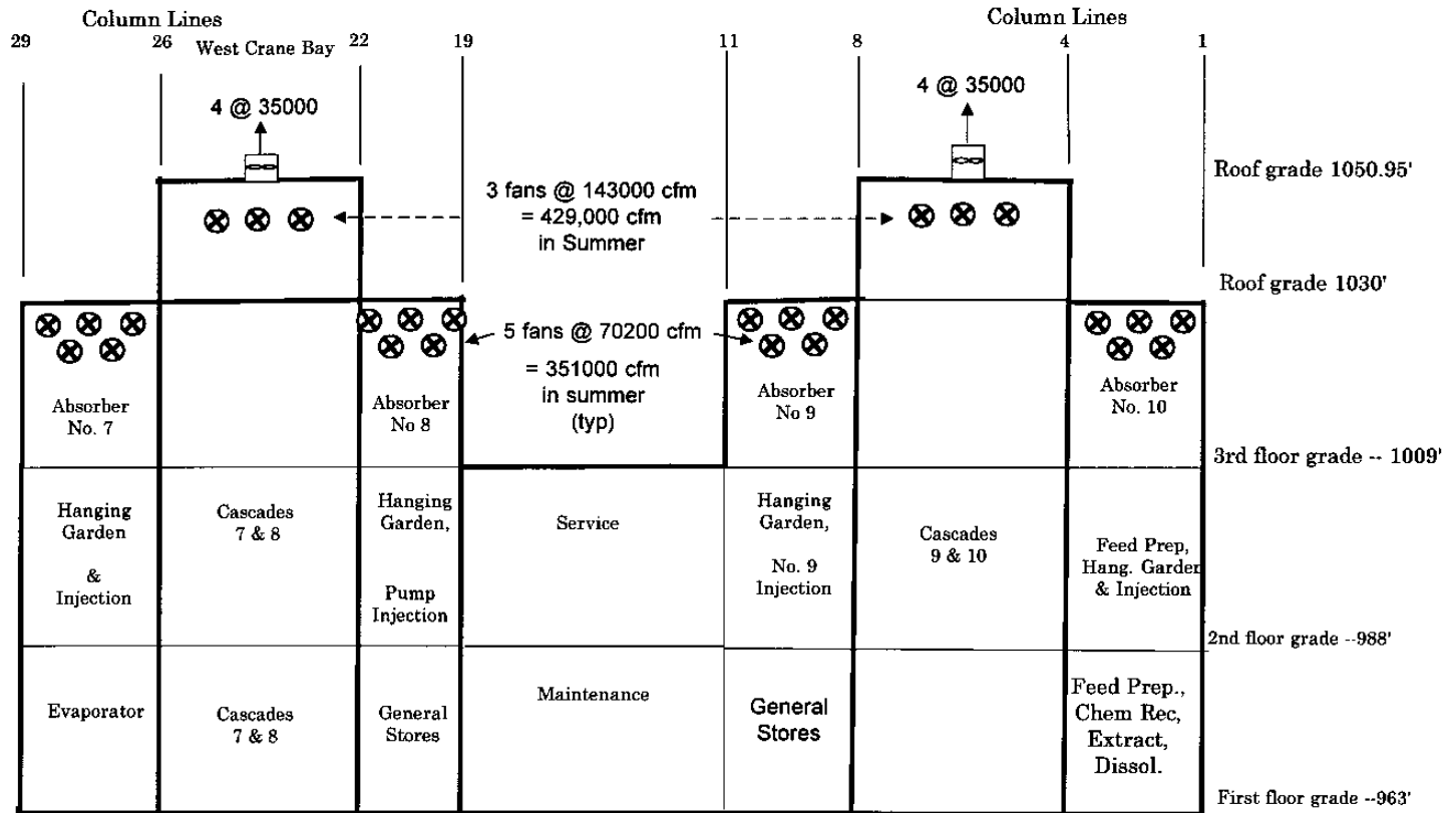
Figure 4 Section A - A (Looking North)---- Building 9201-4
