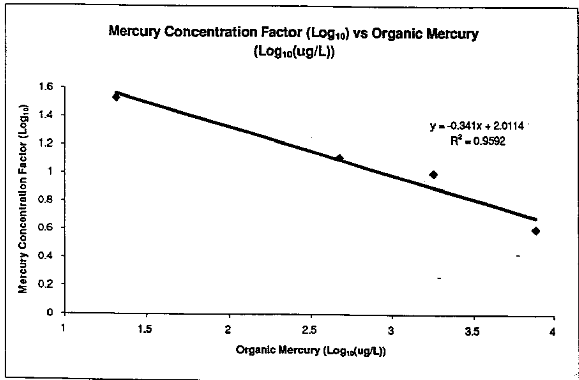
Figure 4. Mercury Concentration Factor in rainbow trout versus inorganic mercury (upper graph) and organic mercury (lower graph), data from Niimi and Kisson (1994).
