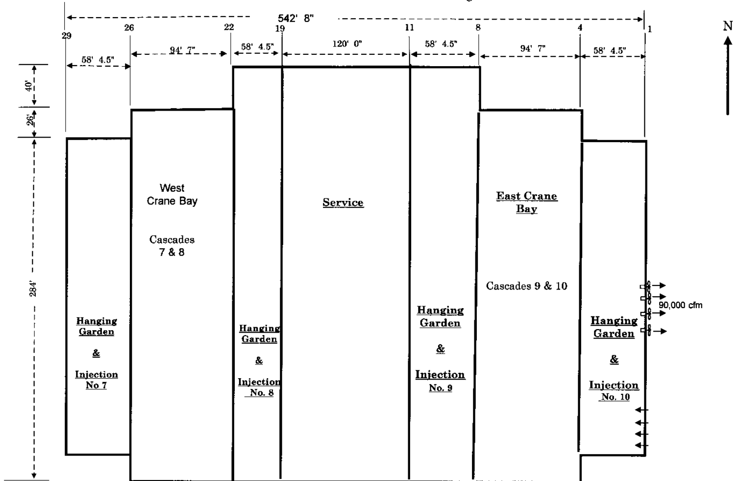
Figure 2 "2nd Floor Plan" -- Building 9201-4
