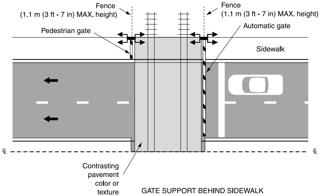
Figure 10D-5. Typical Placement of Pedestrian Traffic Gates
