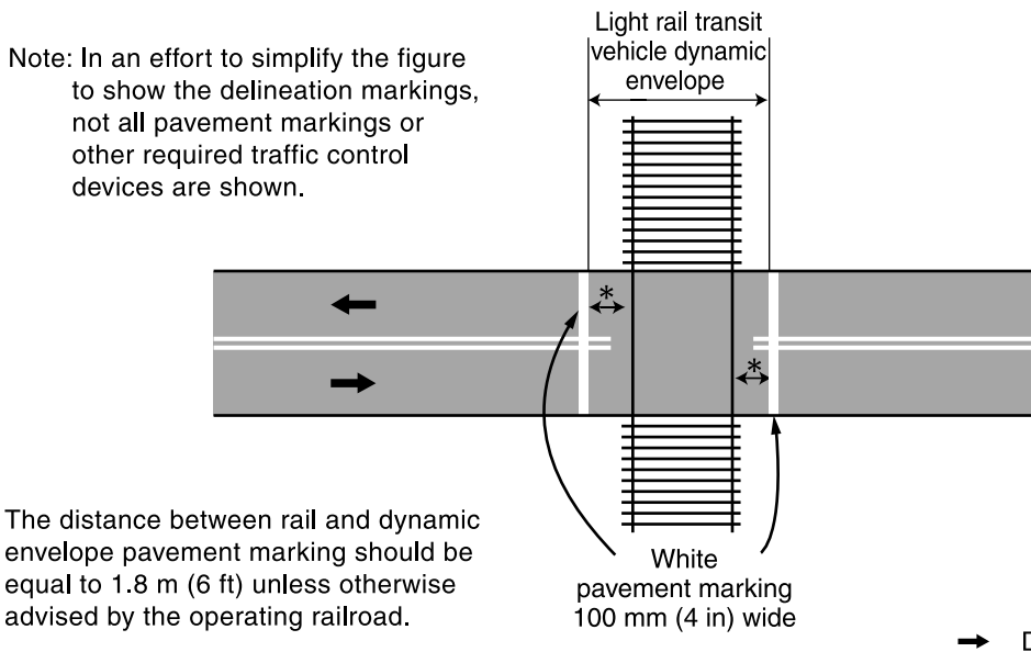
Figure 10C-2. Typical Light Rail Transit Vehicle Dynamic Envelope Delineation Pavement Markings
