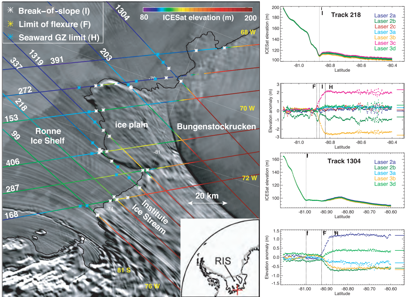
Figure 5. Left panel: Locations of ICESat tracks crossing the region near the entrance of Institute Ice Stream into the southern Ronne Ice Shelf. Tracks are color-coded by elevation relative to the WGS-84 ellipsoid. The background image is the MODIS MOA; the red plus sign on the inset map shows its location in Antarctica; the black line is the break-in-slope from MOA. The asterisks indicate grounding zone features identified from ICESat repeat-track analyses. Right panel: Repeat-track ICESat profiles and elevation anomaly profiles (difference from the mean) for Tracks 218 and 1304 showing features of the grounding zone. Horizontal lines at right are the equivalent anomalies based on tide predictions from a tide model. I is the break-in-slope; F is the limit of flexure, and H is the seaward limit of the grounding zone (GZ). This technique has now been used to map the grounding zone (figure courtesy of Padman and Fricker 2005).
