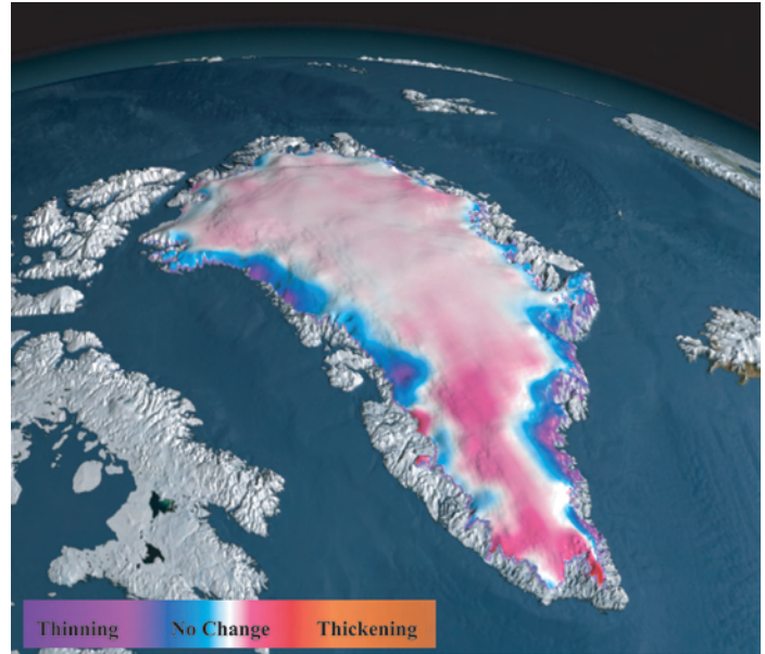
Figure 1. Changes in elevation over the Greenland ice sheet derived from ICESat-I between 2003 and 2006. The pink and red regions indicate a slight thickening, while the blue and purple shades indicate thinning of the ice sheet.
