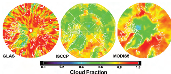
Figure 13. The comparison of the total fraction of clouds detected in the Arctic for October 2003 from GLAS to results for the same period for the International Satellite Cloud Climatology Project and the current MODIS cloud retrieval. The greater sensitivity and discrimination of the laser sensing results in much greater detection for clouds of optical thickness less than 0.2 (figure courtesy of James Spinhirne).
