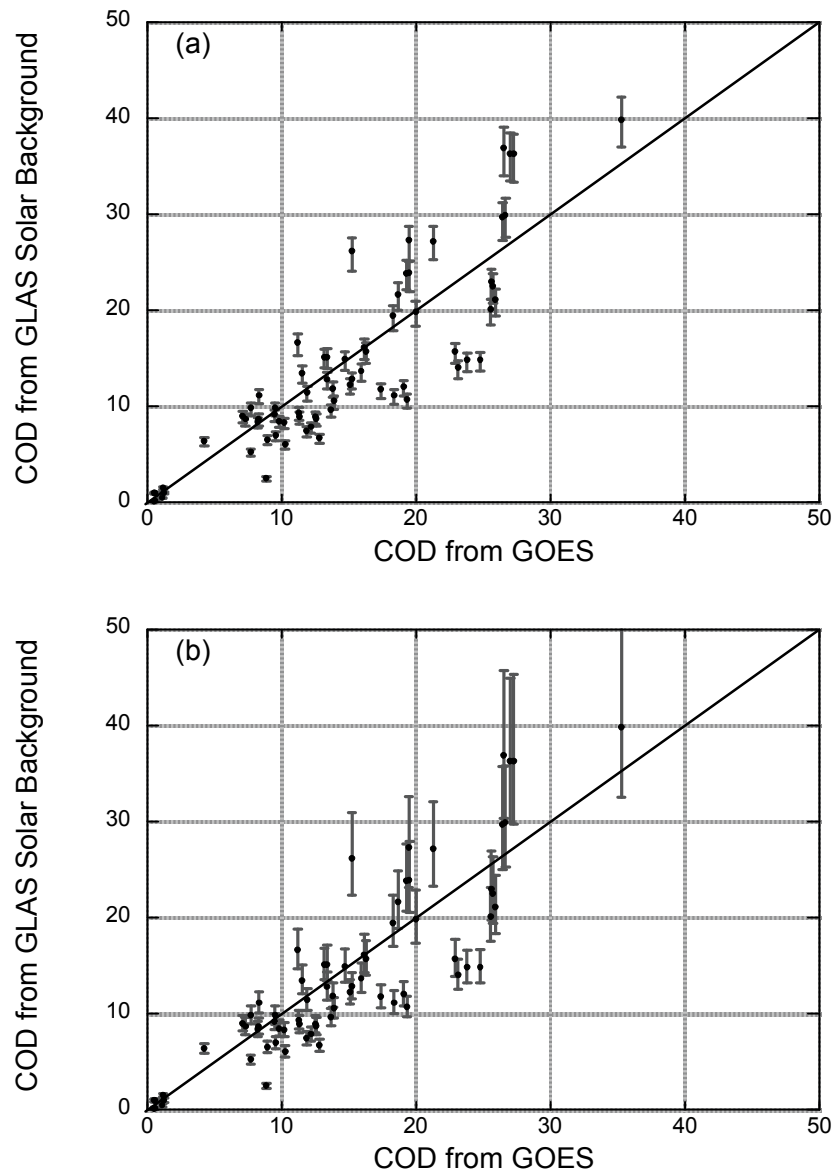
Fig. 12. Same as Fig. 11b, except the possible errors of retrievals from the GLAS 532 nm are also shown. (a) Errors resulted from the uncertainty in droplet effective radius (from 6 \mu\text{m} to 16 \mu\text{m} ) and (b) errors resulted from the uncertainty in calibration coefficient (5%).
