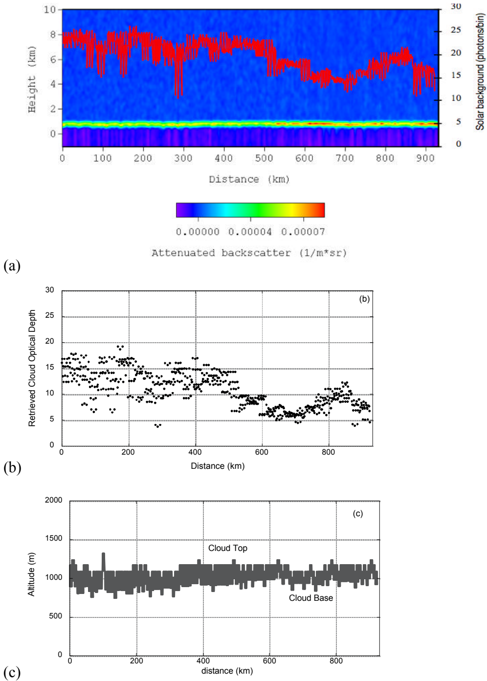
Fig. 14. A marine stratocumulus scene over the southern Pacific Ocean observed on November 1 st , 2003, (a) GLAS 532 nm backscattering image and the corresponding solar background photon counts in the unit of Photons/bin; (b) COD retrieved from GLAS 532 nm solar background at resolution 0.2 sec (1.4 km)); and (c) cloud top observed by GLAS mapped to the same resolution as in panel (b) and cloud base derived from an empirical equation (Minnis et. al. 1992).
