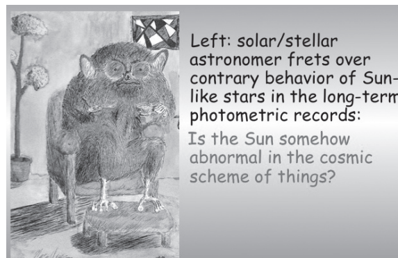
Figure 8. There are many ambiguities between solar and stellar photometric records that inhibit reliable determination of the stellar context of solar variability. Credit: T. Ayres.
