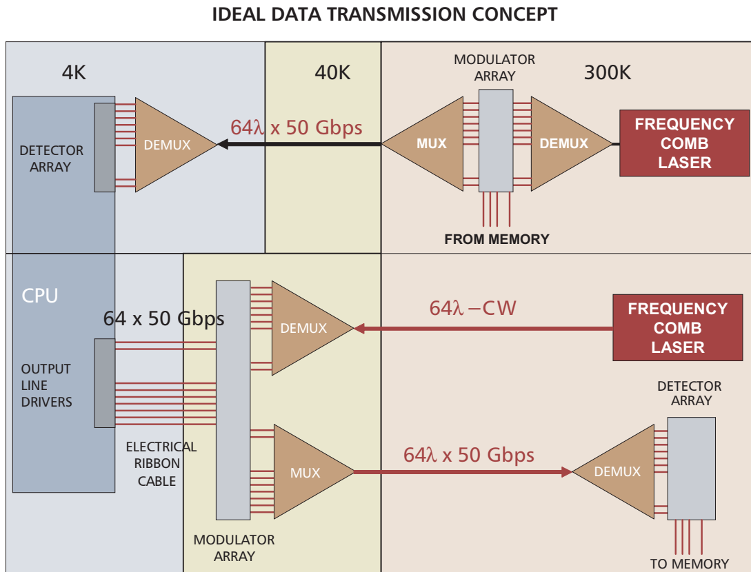
Figure 5. A 3-fiber, 64-wavelength, 50-Gbps DWDM System for bidirectional transmission totaling 6.4 Tbps between a superconductive processor at 4 K and high speed mass memory at 300K. Optical connections are shown in red, electrical in black.
