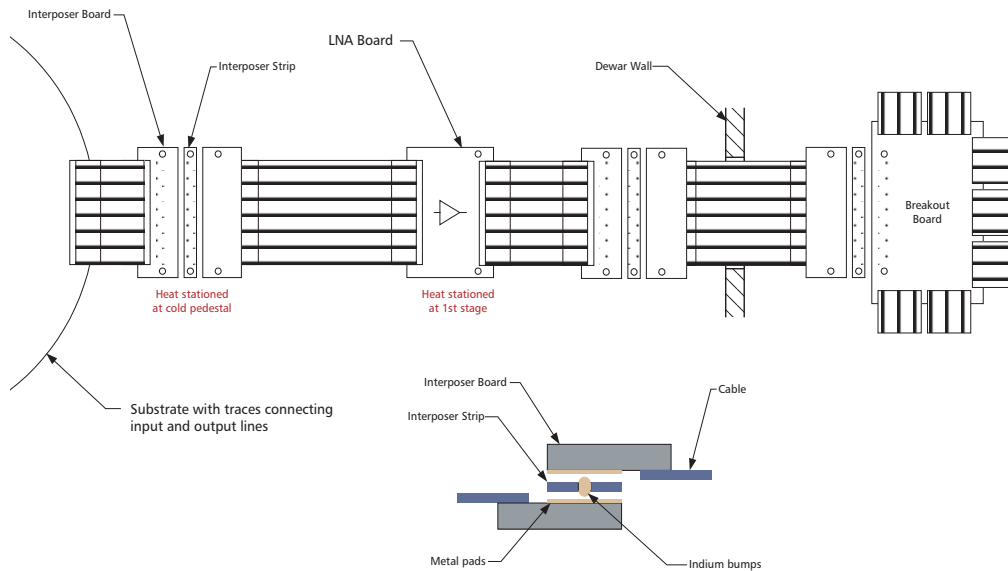
Figure 12. A high-speed flexible ribbon cable designed for modular attachment (Ref: NGST).
