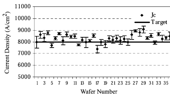
Fig. 3. Trend chart of current density ( J_c ). Mean = 8.3 ± 0.37 kA/cm 2 or ±4.4% (1σ). Target specification = 8.0 kA/cm 2 ± 10% (1σ).
