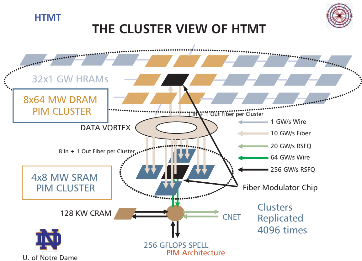
Figure 2. Long path data signal transmission requirements for one proposed petaflop architecture. This would require over 500,000 data channels at 50 Gbps each, assuming 64 bit words.
