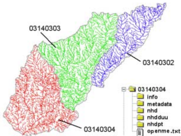
Figure 1. Example NHD data for three subbasins.
