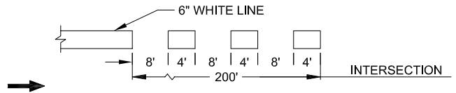
DETAIL 39A
