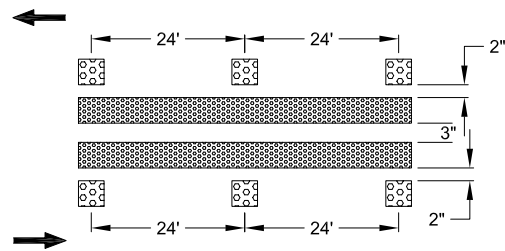
DETAIL 22
