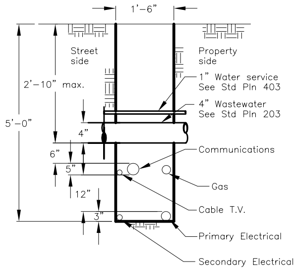
Trench Section
