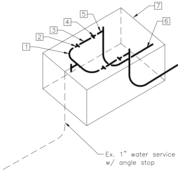
Water Service
