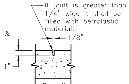
Detail Weakened Plane Joint
