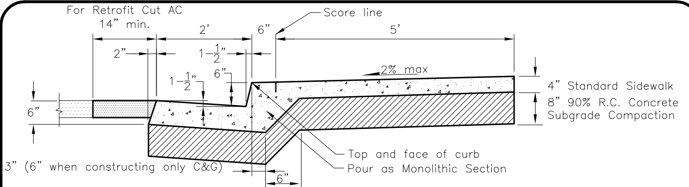
Curb, Gutter, & Sidewalk Section
