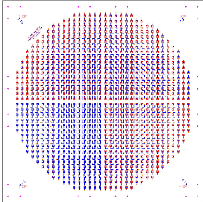
Fig. 1. Layout of the 952 antenna elements of both front-end array (red) and feed-side array (blue) that compose the SFL. Front-end antennas are RHCP polarized because of the incoming signal, and feed-side antennas are linearly polarized for design simplicity and reducing inter-element coupling.
