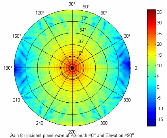
Gain for incident plane wave at Azimuth = 0^\circ and Elevation = 90^\circ
