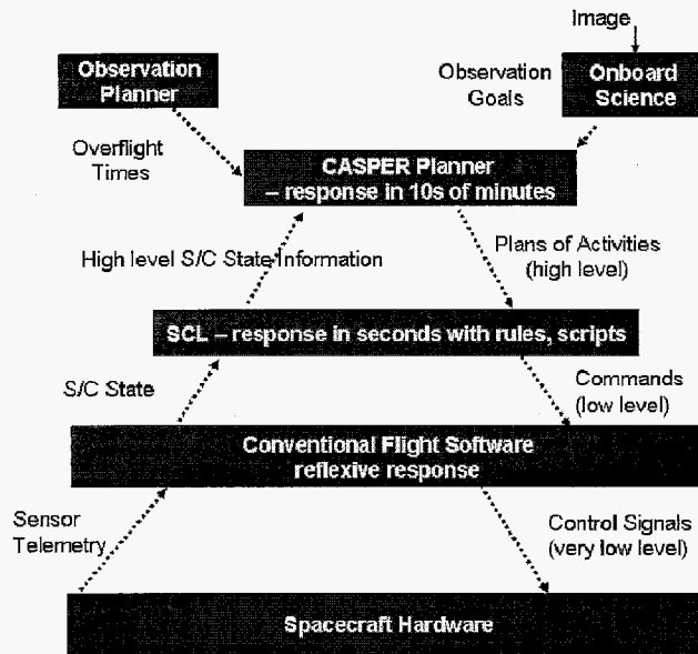
Figure 1. Autonomy Software Architecture
