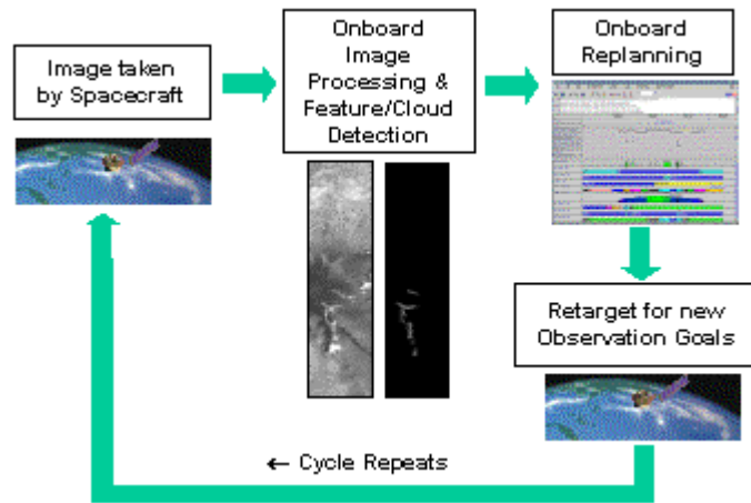
Figure 1. Autonomous Science Mission Concept
