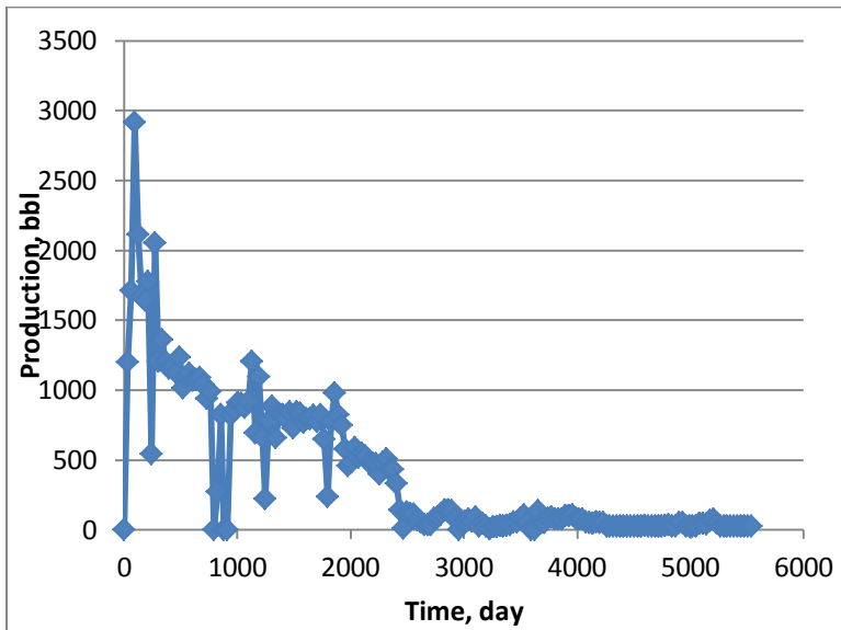
Figure K6. Oil production from well RA1
