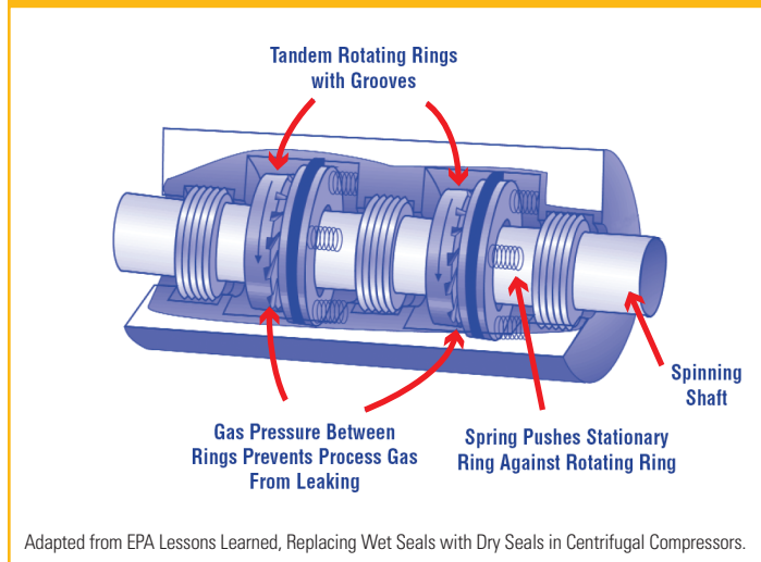
Figure 21: Centrifugal Compressor Dry Seals
