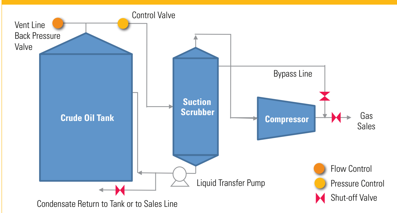
Figure 32: Vapor Recovery Unit Schematic
