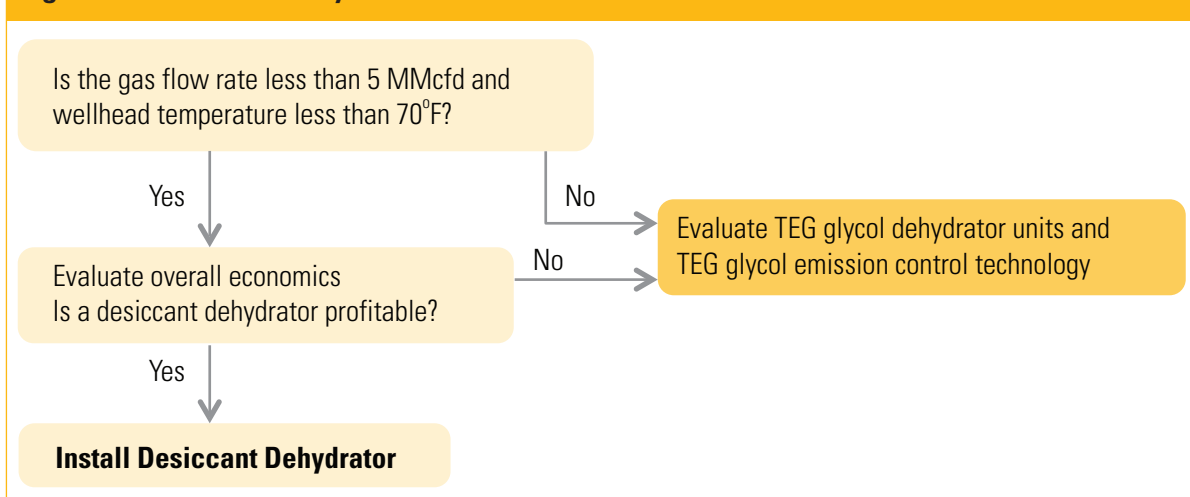
Figure 19: Desiccant Dehydrator Evaluation Flowchart
