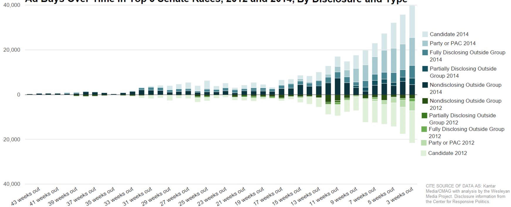
Ad Buys Over Time in Top 5 Senate Races, 2012 and 2014, By Disclosure and Type
