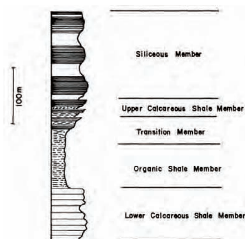
Figure 4-8. Generalized stratigraphic section of the Monterey Formation from the Santa Barbara coastal region (Isaacs, 1980). Open pattern depicts massive units, broken stipple indicates irregularly laminated beds, and thinly lined pattern denotes finely laminated units.
