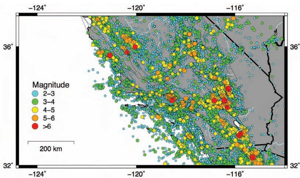
Figure 5-9. High-precision earthquake locations 1981-2011 from Hauksson et al. (2011). Faults as in Figure 5-8.
