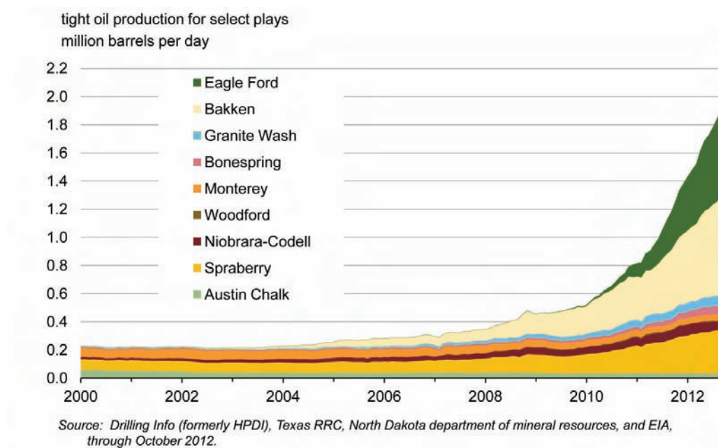
Figure 1-1. Oil production through time from selected low permeability (“tight”) oil plays in the United States US EIA (2013).
