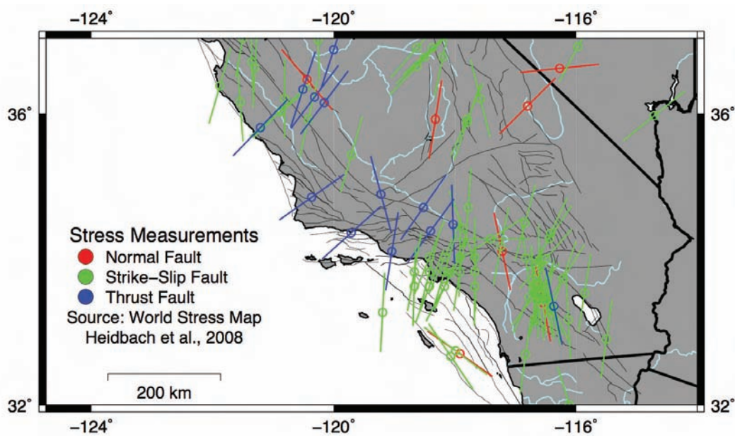
Figure 5-8. Highest quality stress measurements for California from the World Stress Map (Heidbach et al., 2008), plotted with mapped faults from UCERF3 FM 3.1 (Field et al., 2014). Stress measurements show orientation of the maximum horizontal compressive stress direction, color-coded according to stress regime.
