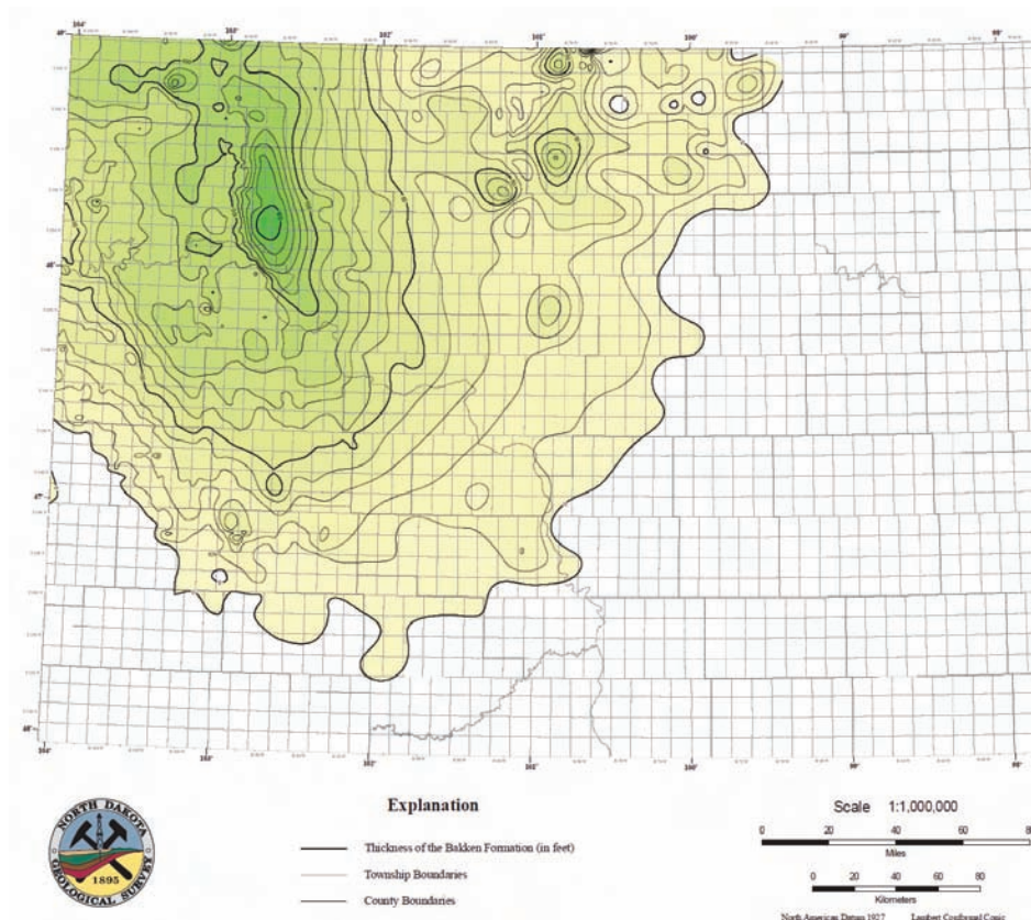
Figure 4-15. Isopach map of the Bakken Formation (Lefever, 2008).
