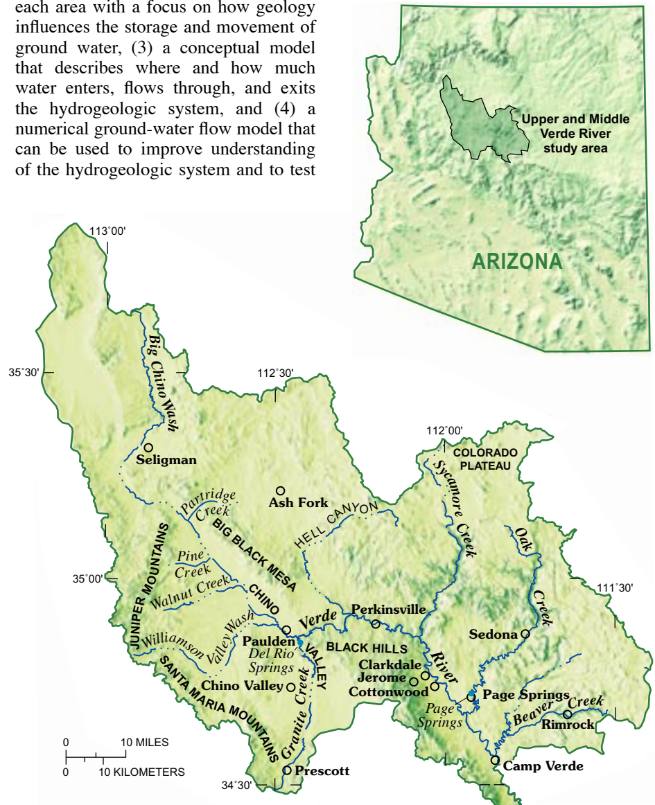
Figure 1. Location of the upper and middle Verde River study area.
